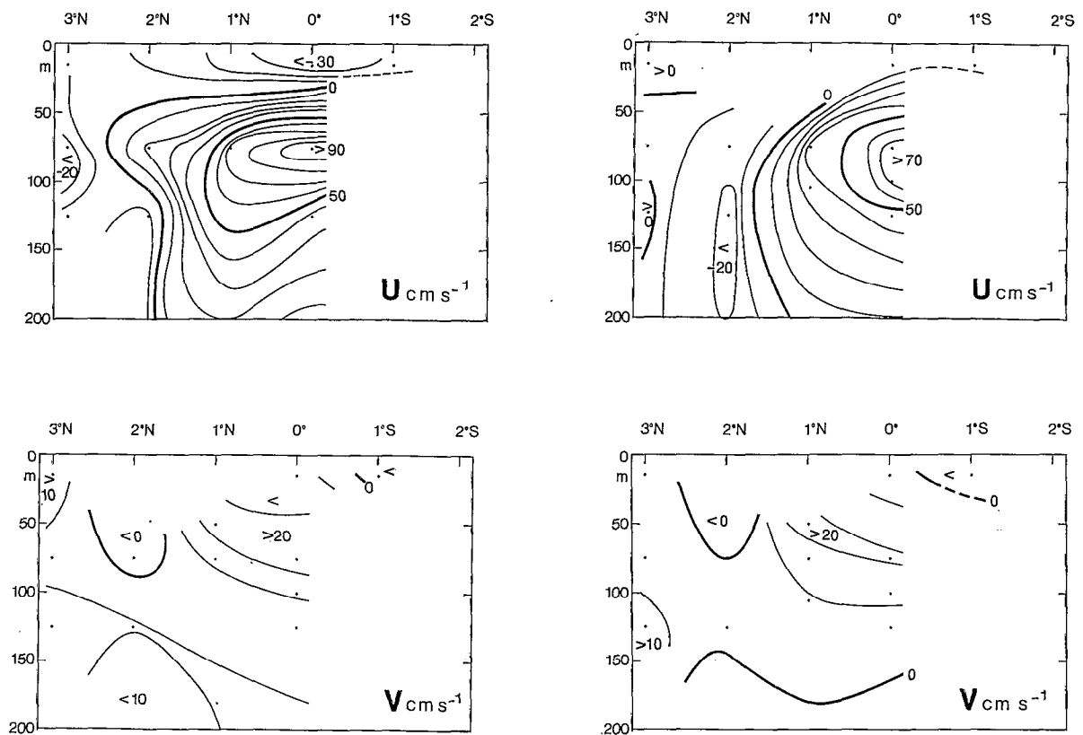
FIG. 7. — The mean currents measured during section 3, 17 to 20 February 1979, left, and section 4, 2 to 6 March 1979, right (u positive to the east, v positive to the north)
