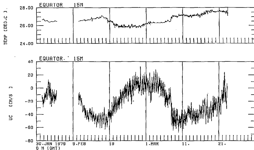
FIG. 6. — Time series of the temperature and the zonal component of the current at the equator at 15 m depth.
