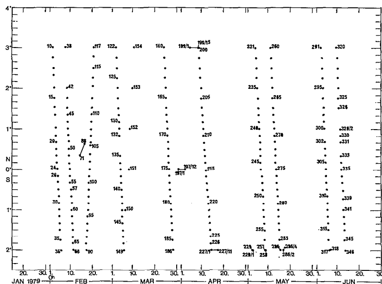
FIG. 2. — The time and meridional distribution of the STD-measurements and nutrient casts
