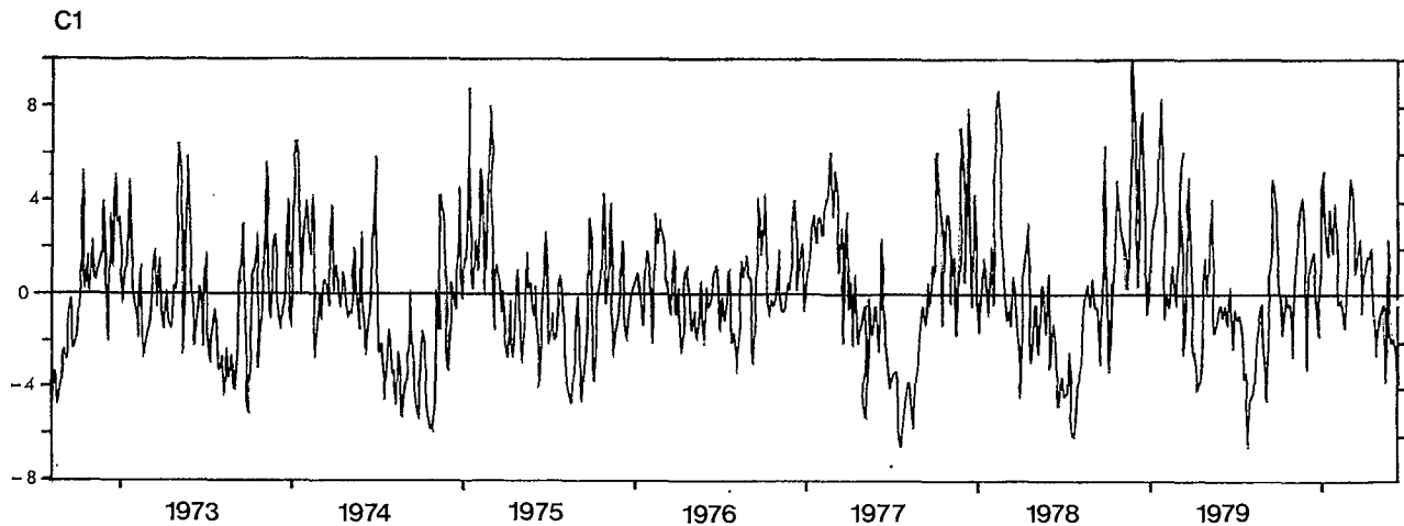
FIG. 8a. - As Fig. 6a for the first EOF shown in Fig. 7c.
