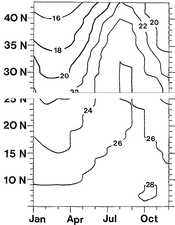
FIG. 2 b. — Monthly mean values of sea surface temperatures,
