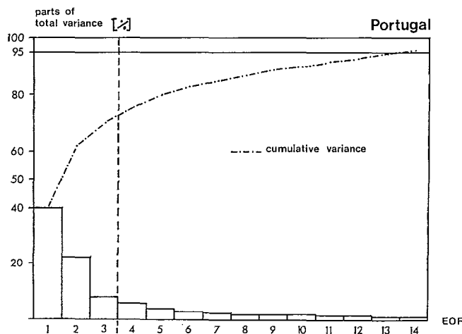
FIG. 8b. - As Fig. 6b for the analysis in the area between 36° N and 43° N.
