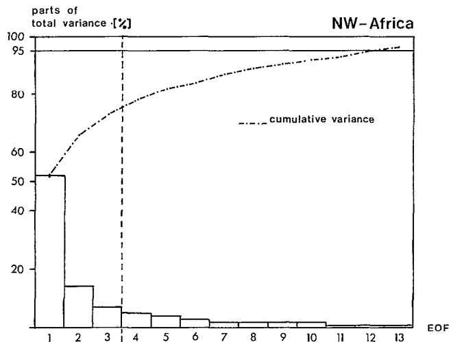
FIG. 6 b. — Histogram explaining the percentage part of each EOF to the total variance, for the analysis in the area between 10^{\circ} N and 22^{\circ} N. The first three EOF's (cf. Fig. 5 c-e) are significant.
