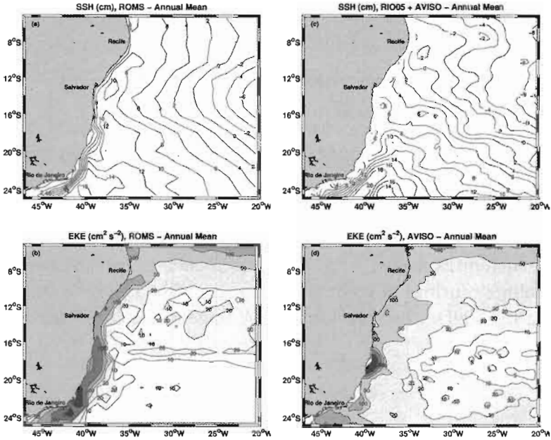
Figure 6 – Averaged (2005-2007) SSH and EKE comparisons between ROMS simulations and AVISO Rio05 data: (a) ROMS - SSH (cm), (b) ROMS - EKE ( \text{cm}^2 \text{s}^{-2} ), (c) RIO05 + AVISO - SSH (cm) and (d) AVISO - EKE ( \text{cm}^2 \text{s}^{-2} ).
