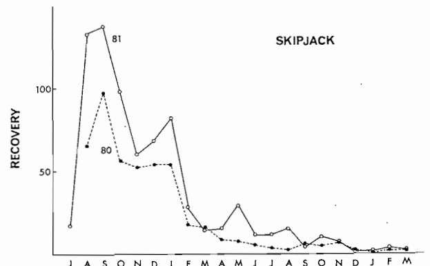
Figure 10. Recoveries by month of skipjack tagged and released in 1980 (broken line) and 1981 (solid line).
