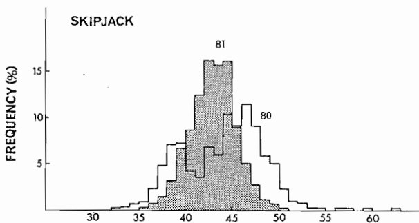
Figure 3. Length frequency distribution of tagged skipjack. The histogram for fish tagged in 1981 is shaded.
