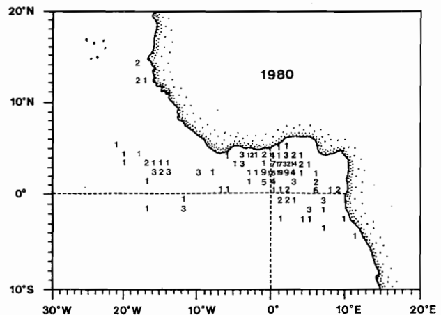
Figure 4. Distribution of the recoveries for tagged skipjack in 1980. Numerals show the number of recoveries by 1° square.
