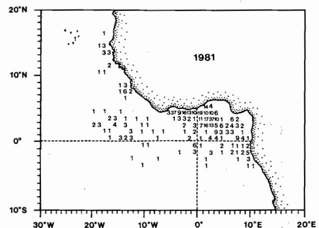
Figure 5. Distribution of the recoveries for tagged skipjack in 1981. Numerals show the number of recoveries by 1° square. Three recoveries were reported from outside this figure at 27°N, 15°W; 14°S, 10°E; and 13°S, 12°E.
