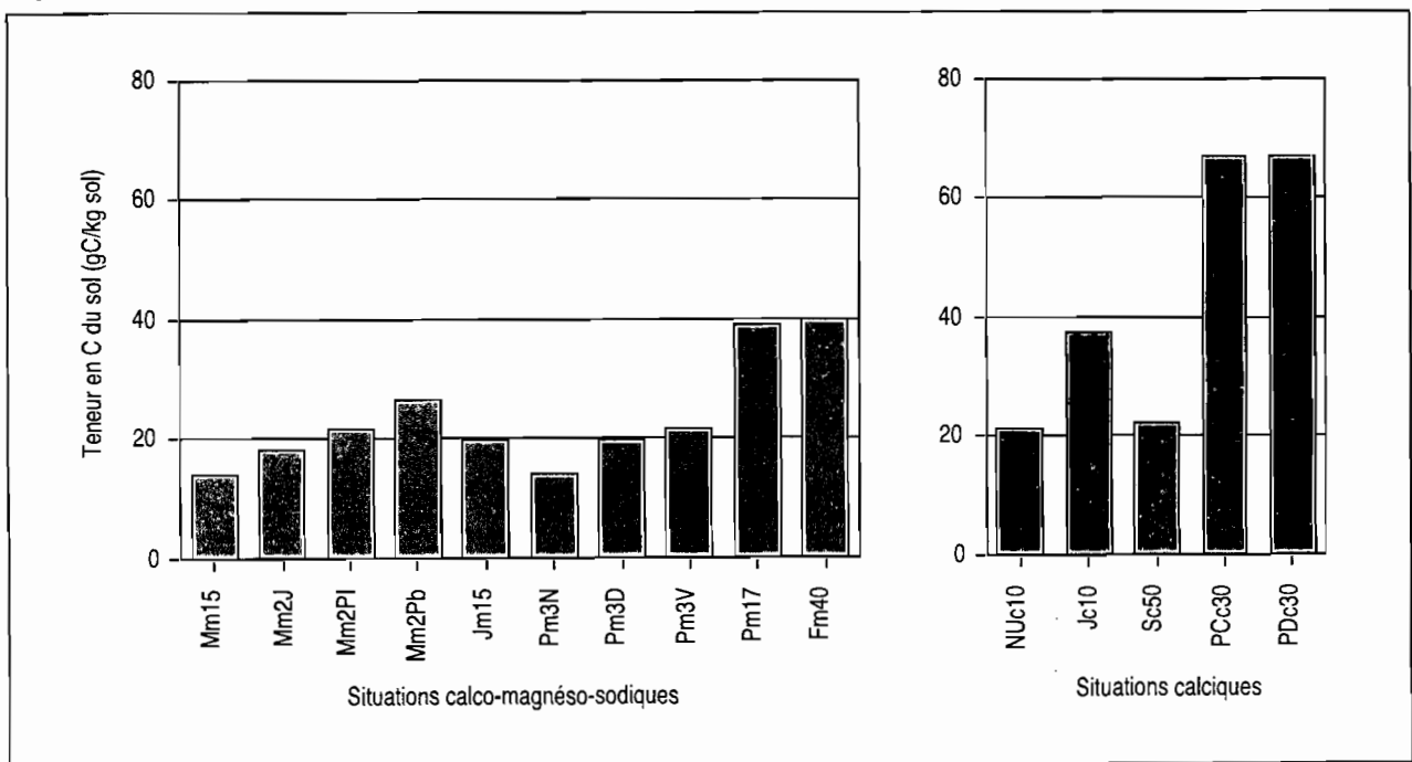
Figure 8 - C contents (g/kg soil) in different situations (0-10 cm depth).
