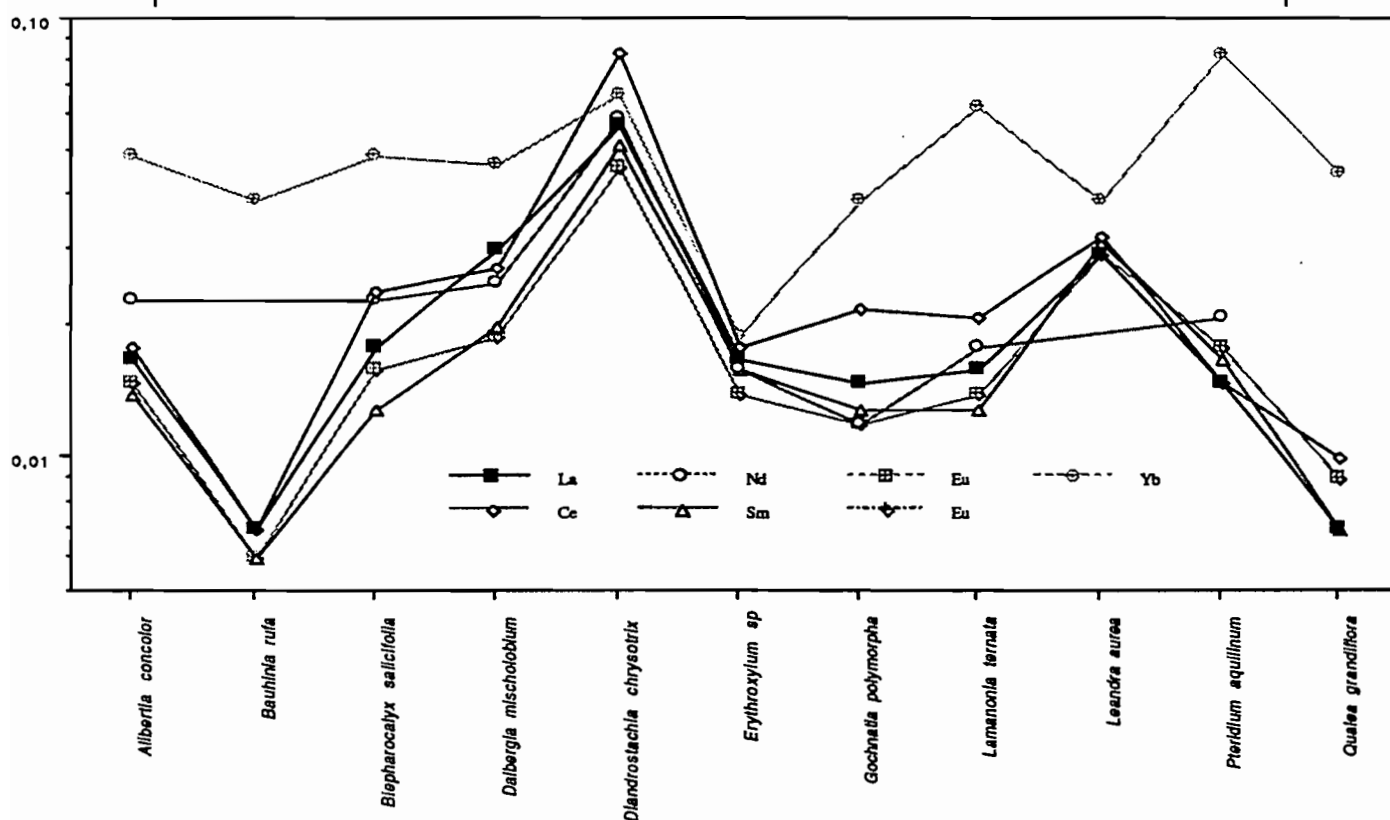
Fig. 2 REE abundance in the different plant species (values normalised to the mean REE abundance in soil samples)
