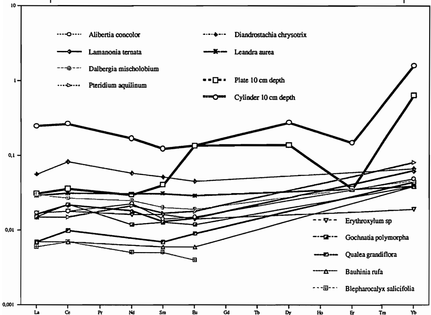
Figure 3- REE abundance in plant and water samples (values normalized to the mean REE abundance in soil samples)
