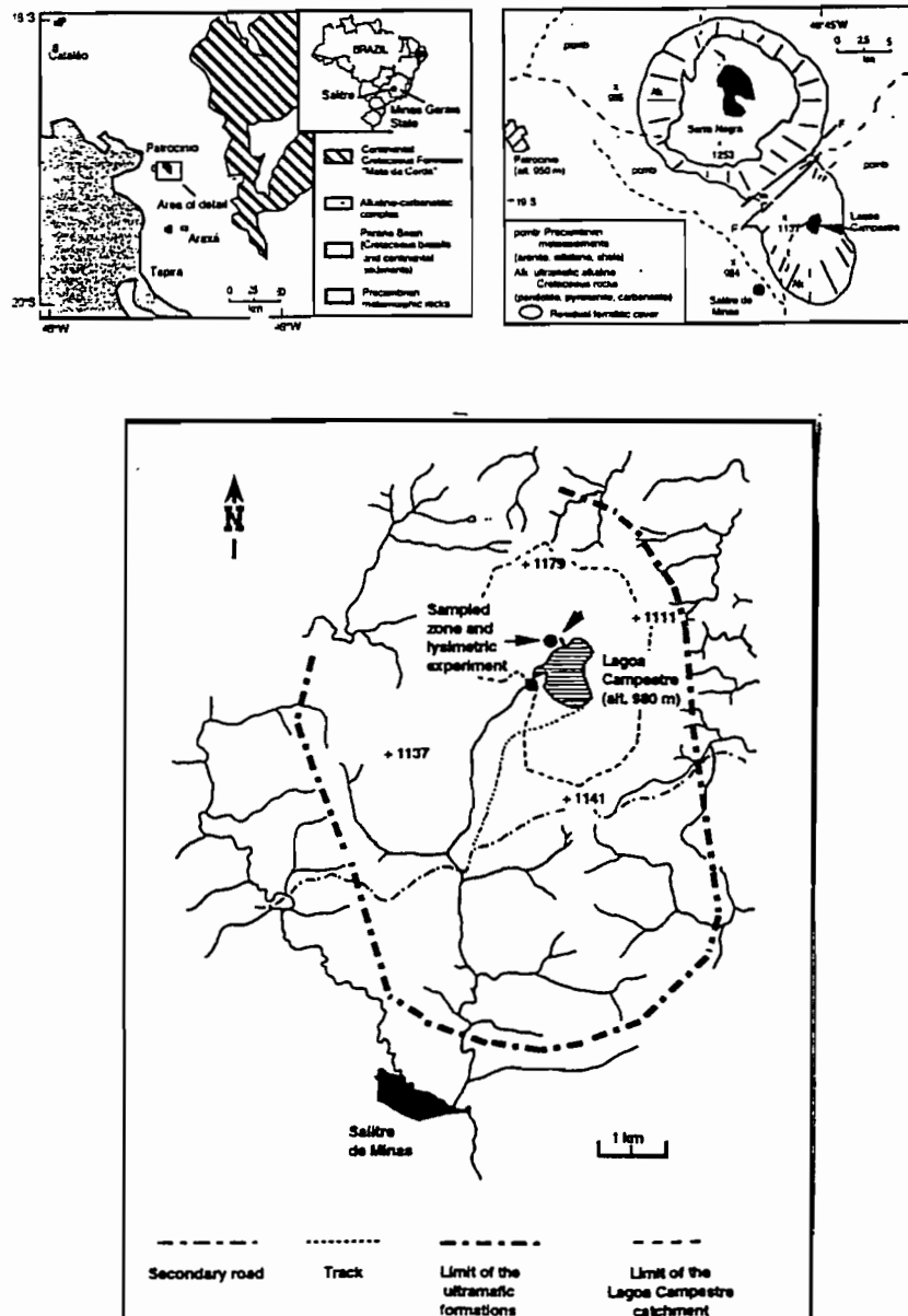
Figure 1: Localisation of the Salitre area, geological context, drainage system and location of sampled zone and of the lysimetric experiment. (+ 1137 = altitude in meters)
