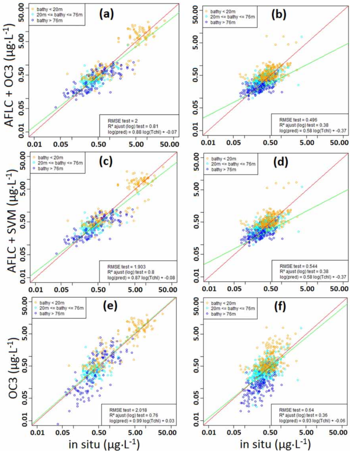
Figure 6. Comparisons of different algorithms on a test sample including data from SeaBASS and data from NCDDataBase (left column) and on NCDDataBase (right column) (a) “AFLC + OC3”; (b) idem on full NCDDataBase; with 3 bathymetry groups (c) “AFLC + SVM”; (d) idem on full NCDDataBase; (e) Result of OC3; (f) Idem on full NCDDataBase; RMSE, R^2_{\text{ajusted}} and the linear regression line between \log(chl - a_{in\ situ}) and \log(chl - a_{algorithm}) . The line y = x is red and the regression line is green.
