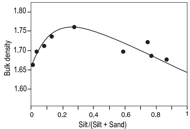
Figure 4. Bulk density recorded by Fiès and Stengel (1981) according to the proportion of silt (20-50 \mu\text{m} ) relative to the silt and sand particles (200-2,000 \mu\text{m} ) in soils with clay content <20% and no macroporosity
