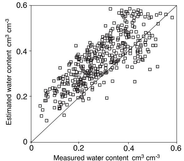
Figure 6. Comparison between measured values of volumetric water content at -33 kPa water potential and those estimated by the pedotransfer functions of Rawls et al. (1982) (modified after Tomasella and Hodnett, 1998)
