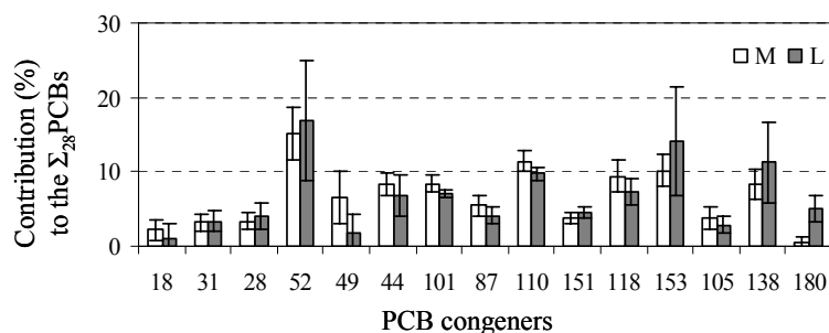
Figure 1. PCB patterns in the muscle (M) and liver (L) of yellowfin tunas (n=5) from the western Indian Ocean. Mean values ( \pm standard deviation) of the contribution of each congener to the \Sigma_{28} PCBs.
