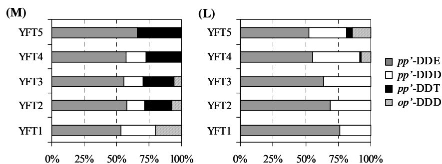
Figure 2. Composition of DDTs in the muscle (A) and liver (B) of yellowfin tunas (YFT, n=5) from the western Indian Ocean.
