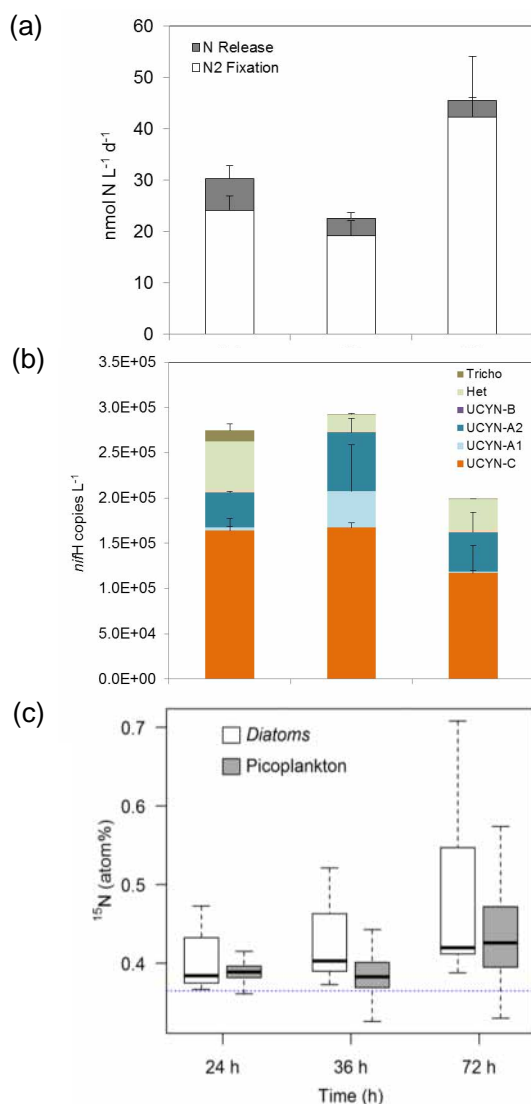
Figure 5. Results from the DDN transfer experiment performed from day 17 to 20 in M2. (a) Temporal changes in 15 N 2 uptake (white, nmol N L -1 d -1 ) and quantification of DDN in the dissolved pool (grey) over the course of the experiment. Error bars represent the standard deviation of three independent replicate incubations. (b) Temporal changes in diazotroph abundance determined by qPCR ( ni/H gene copies L -1 ) during the same experiment. Error bars represent the standard deviation of triplicate incubations. (c) Summary of the nanoSIMS analyses. Measured 13 C and 15 N at. % values of non-diazotrophic diatoms (white) and picoplankton (grey) as a function of incubation time. The horizontal dashed line indicates the natural abundance of 15 N (0.366 at. %), and the error bars represent the standard deviation for the several cells analyzed by nanoSIMS.
