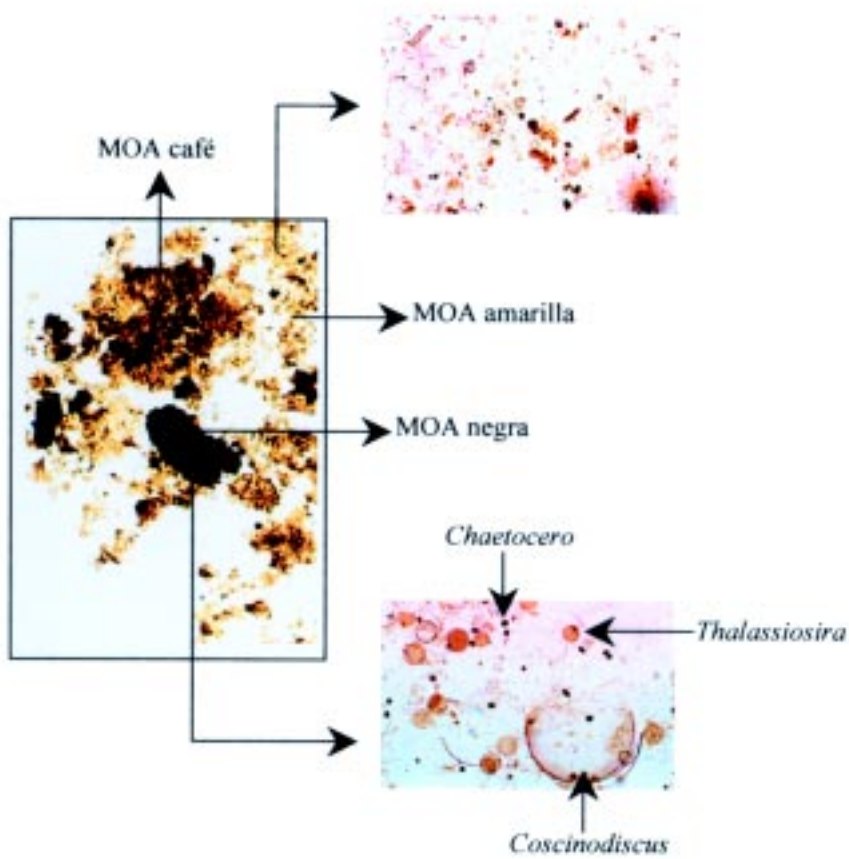
Fig. 3: Características de la materia orgánica vista en el microscopio de luz transmitida. Major characteristics of the organic matter as viewed in a transmitted-light microscope.
