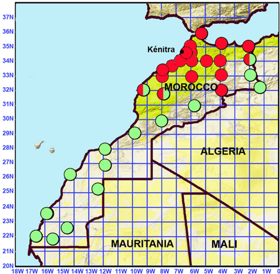
Figure 1. Geographic distribution of Ornithodoros erradicus s.s. (red circles) and O. sonrai (light green circles). doi:10.1371/journal.pntd.0001810.g001
