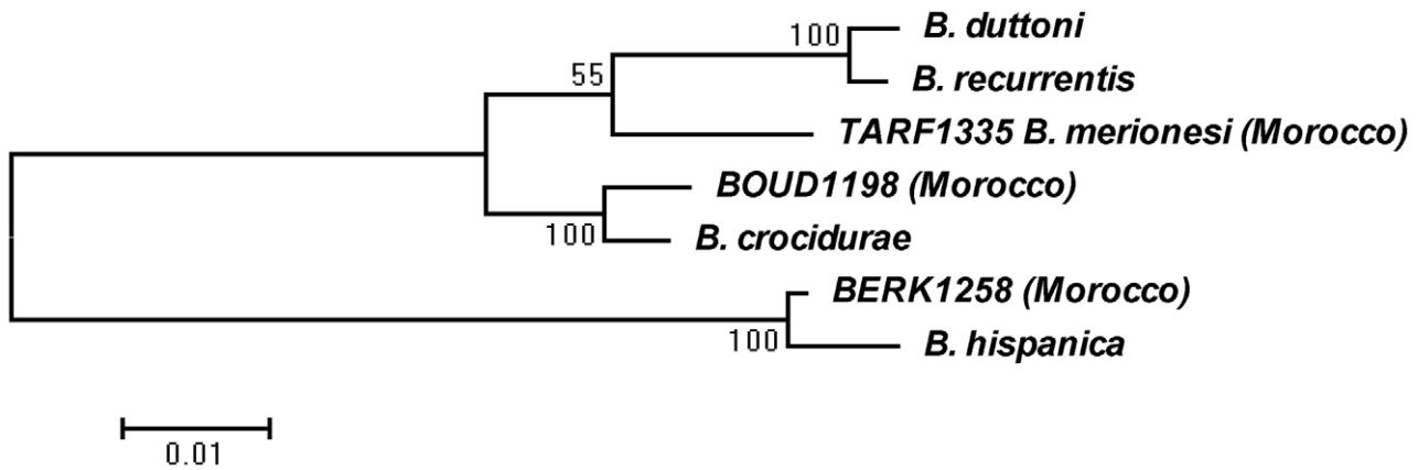
Figure 3. Phylogenetic relationships among Borrelia species in Morocco. doi:10.1371/journal.pntd.0001810.g003
