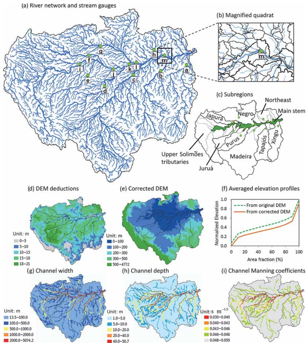
Figure 2. Basin discretization and model inputs. (a) The river network extracted from the DEM overlaps with 13 stream gauges: (a) Altamira; (b) Itaituba; (c) Fazenda Vista Alegre; (d) Canutama; (e) Gavião; (f) Acanai; (g) Serrinha; (h) Cachoeira da Porteira; (i) Santo Antônio do Içá; (j) Itapeua; (k) Manacapuru; (l) Jatuarana and Careiro; (m) Óbidos. Panel (b) indicates the magnified quadrat. The thin (thick) black lines mark boundaries between subbasins (subregions). Panel (c) indicates the delineation of 10 subregions (including 9 tributary subregions and the main stem subregion indicated by dark green color). Panel (d) indicates average DEM deductions at each subbasin for alleviating vegetation-caused biases; (e) the corrected DEM; (f) averaged elevation profiles based on the original and corrected DEMs; (g) channel widths; (h) channel depths; and (i) Manning roughness coefficients of channels.
