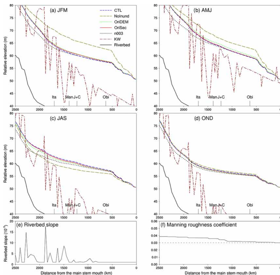
Figure 10. Modeled average river surface profiles along the middle and lower main stem in the four seasons of the year 2005: (a) JFM (January, February and March; the period of rising flood); (b) AMJ (April, May and June; the period of high water); (c) JAS (July, August and September; the period of falling flood); and (d) OND (October, November and December; the period of low water). Results of six simulations are shown. The four stream-gauge locations are labeled on the x axis: Ita – Itapeua; Man – Manacapuru; J+C – Jatuarana and Careiro; Obi – Óbidos. Riverbed slopes (e) and Manning roughness coefficients (f) along the main stem are also shown. In the panel (f) , the solid curve shows spatially varying Manning coefficients used in five simulations; the dotted line shows the uniform Manning coefficient of 0.03 used in the simulation n003.
