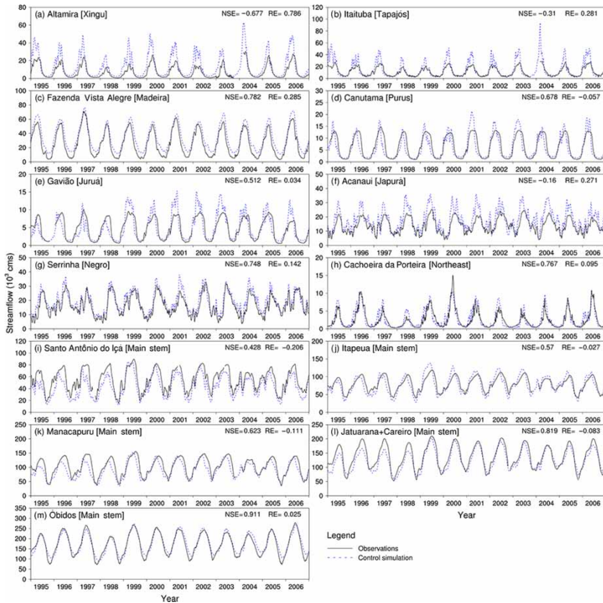
Figure 3. Comparison between modeled and observed daily streamflow for a 12-year period (1995–2006) at 13 stream gauges (the corresponding subregion names are shown in the brackets): (a) Altamira (Xingu); (b) Itaituba (Tapajós); (c) Fazenda Vista Alegre (Madeira); (d) Canutama (Purus); (e) Gavião (Juruá); (f) Acanai (Japurá); (g) Serrinha (Negro); (h) Cachoeira da Porteira (northeast); (i) Santo Antônio do Içá (main stem); (j) Itapeua (main stem); (k) Manacapuru (main stem); (l) Jatuarana and Careiro (main stem); (m) Óbidos (main stem). The Nash–Sutcliffe efficiency coefficient and the relative error of mean annual streamflow are indicated at the upper right corner of each panel. Figure 2a shows the stream-gauge locations.
