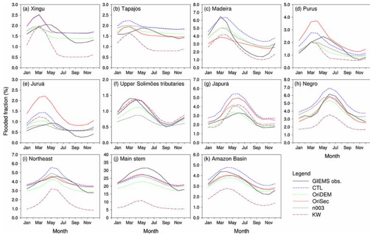
Figure 11. Observed and modeled average monthly flood extent of 13 years (1995–2007) for the 10 subregions and the entire Amazon Basin. Setup of the five simulations is described in Table 2: CTL – control simulation; OriDEM – using the original DEM (with vegetation-caused biases); OriSec – using basin-wide channel geometry formulae; n003 – using a uniform Manning roughness coefficient (i.e., 0.03) for all the channels; KW – using the kinematic wave method to represent river flow.
