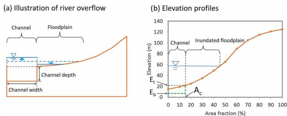
Figure 1. Illustrations of the macroscale inundation scheme: (a) illustration of river overflow; (b) elevation profiles of a computation unit (e.g., a grid cell or subbasin). The brown solid line is the original elevation profile. The green dashed line is the amended elevation profile (its non-channel part overlaps with the original elevation profile). A_c is the fraction of the channel area in the computation unit, E_t is the bank top elevation and E_b is the channel bed elevation.
