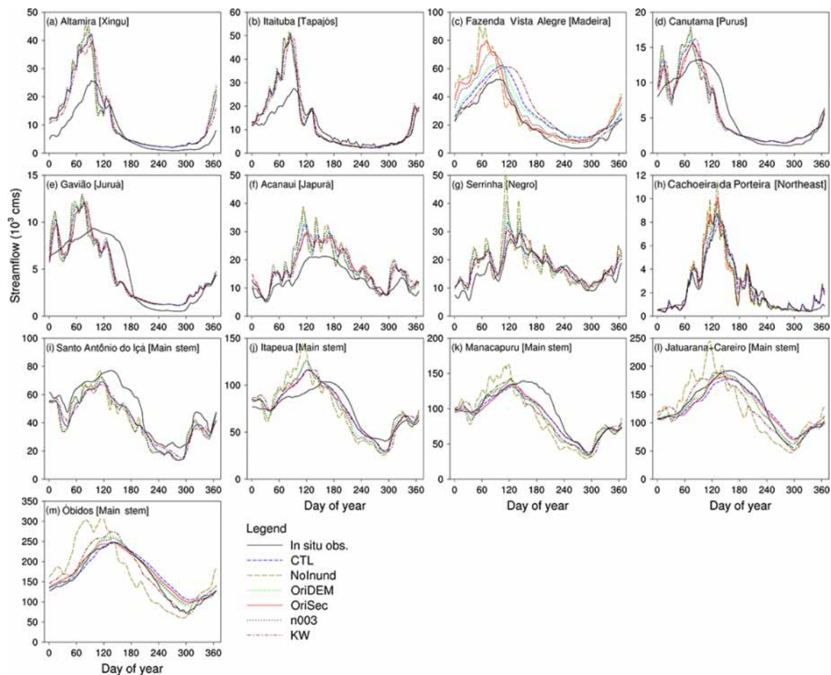
Figure 8. Observed and modeled daily streamflow of the year 2005 at 13 stream gauges. The setup of the six simulations is described in Table 2: CTL – control simulation; NoInund – without inundation scheme; OriDEM – using the original DEM (with vegetation-caused biases); OriSec – using basin-wide channel geometry formulae; n003 – using a uniform Manning roughness coefficient (i.e., 0.03) for all the channels; KW – using the kinematic wave method to represent river flow.
