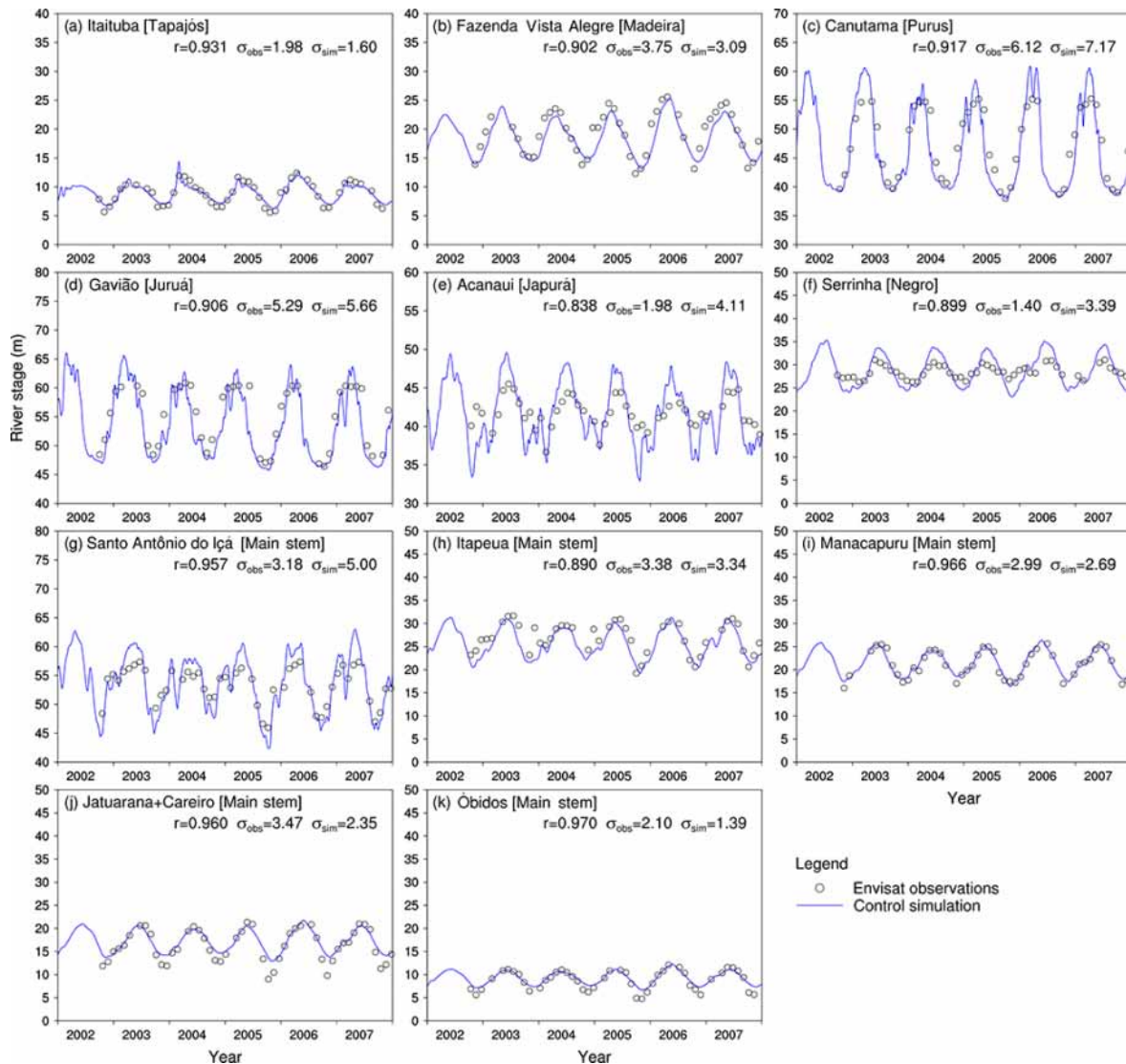
Figure 4. Comparison of modeled daily river stages with the observations for a 6-year period (2002–2007) at the subbasins containing or close to 11 of the 13 stream gauges (the corresponding subregion names are shown in the brackets): (a) Itaituba (Tapajós); (b) Fazenda Vista Alegre (Madeira); (c) Canutama (Purus); (d) Gavião (Juruá); (e) Acanauí (Japurá); (f) Serrinha (Negro); (g) Santo Antônio do Içá (main stem); (h) Itapeua (main stem); (i) Manacapuru (main stem); (j) Jatuarana and Careiro (main stem); (k) Óbidos (main stem). The Pearson correlation coefficient between modeled river stages and the observations, as well as standard deviation for modeled and observed river stages, is indicated in each panel. The simulated river stages are shifted to coincide with the observations for better visual comparison (please see Sect. 3.2 for the detailed explanation).
