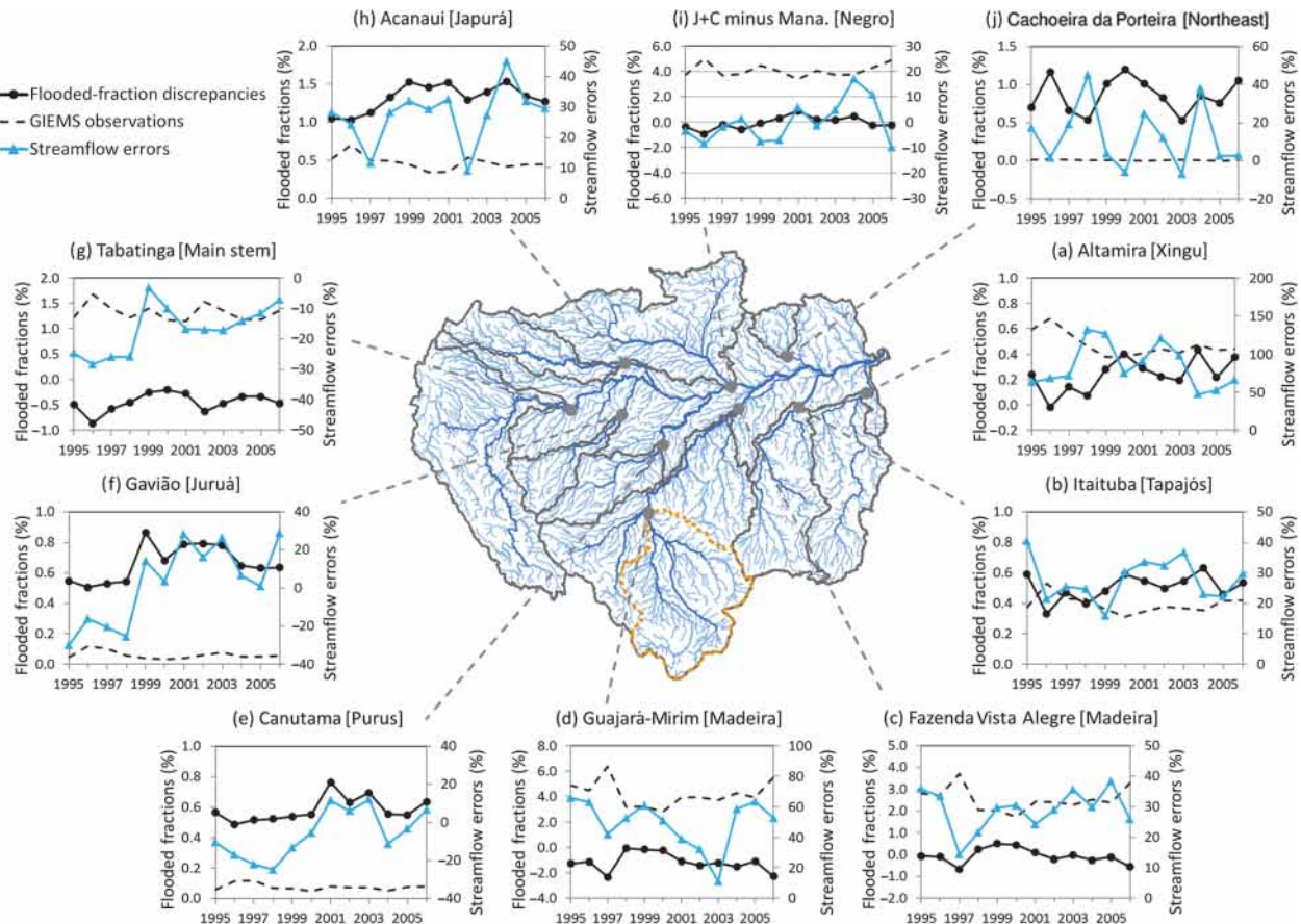
Figure 7. Streamflow errors and the flood extent discrepancies (i.e., the differences between simulated flood extent and the GIEMS data) in the area upstream of the gauge for 10 gauges at the annual scale during 12 years (1995–2006). Streamflow of the Negro subregion (i) is approximated by the streamflow difference between the Jatuarana and Careiro gauge and the Manacapuru gauge. The upstream area of each gauge is enclosed by the gray lines (or brown dotted lines for the Guajará-Mirim gauge) in the basin map.
