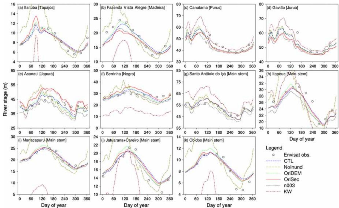
Figure 9. Observed and modeled river stages at the daily scale in the year 2005 for the subbasins containing or close to 11 of the 13 stream gauges. The setup of the six simulations is described in Table 2: CTL – control simulation; NoInund – without inundation scheme; OriDEM – using the original DEM (with vegetation-caused biases); OriSec – using basin-wide channel geometry formulae; n003 – using a uniform Manning roughness coefficient (i.e., 0.03) for all the channels; KW – using the kinematic wave method to represent river flow.
