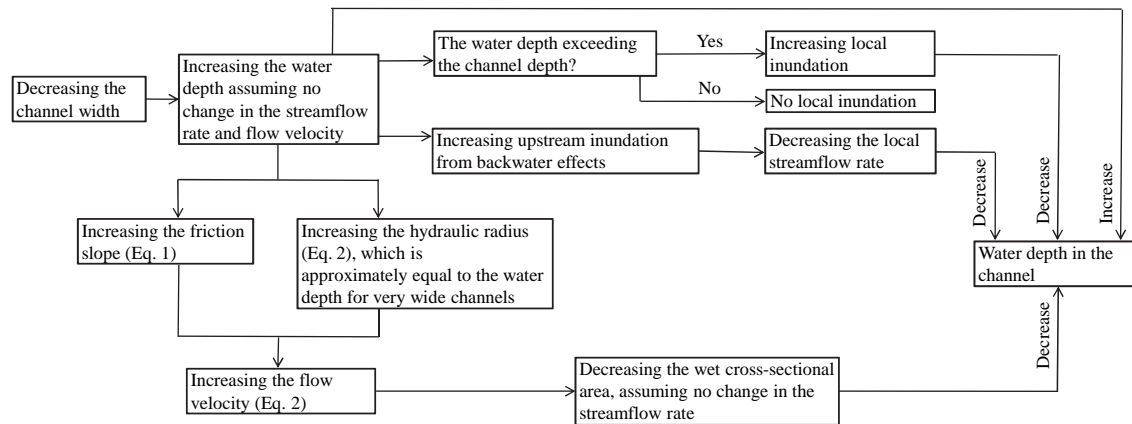
Figure 13. A diagram illustrating that decreasing the width of the local channel could bring about changes in the water depth of the local channel through various mechanisms. In general, the phenomena before and after an arrow have the cause–effect relationship.
