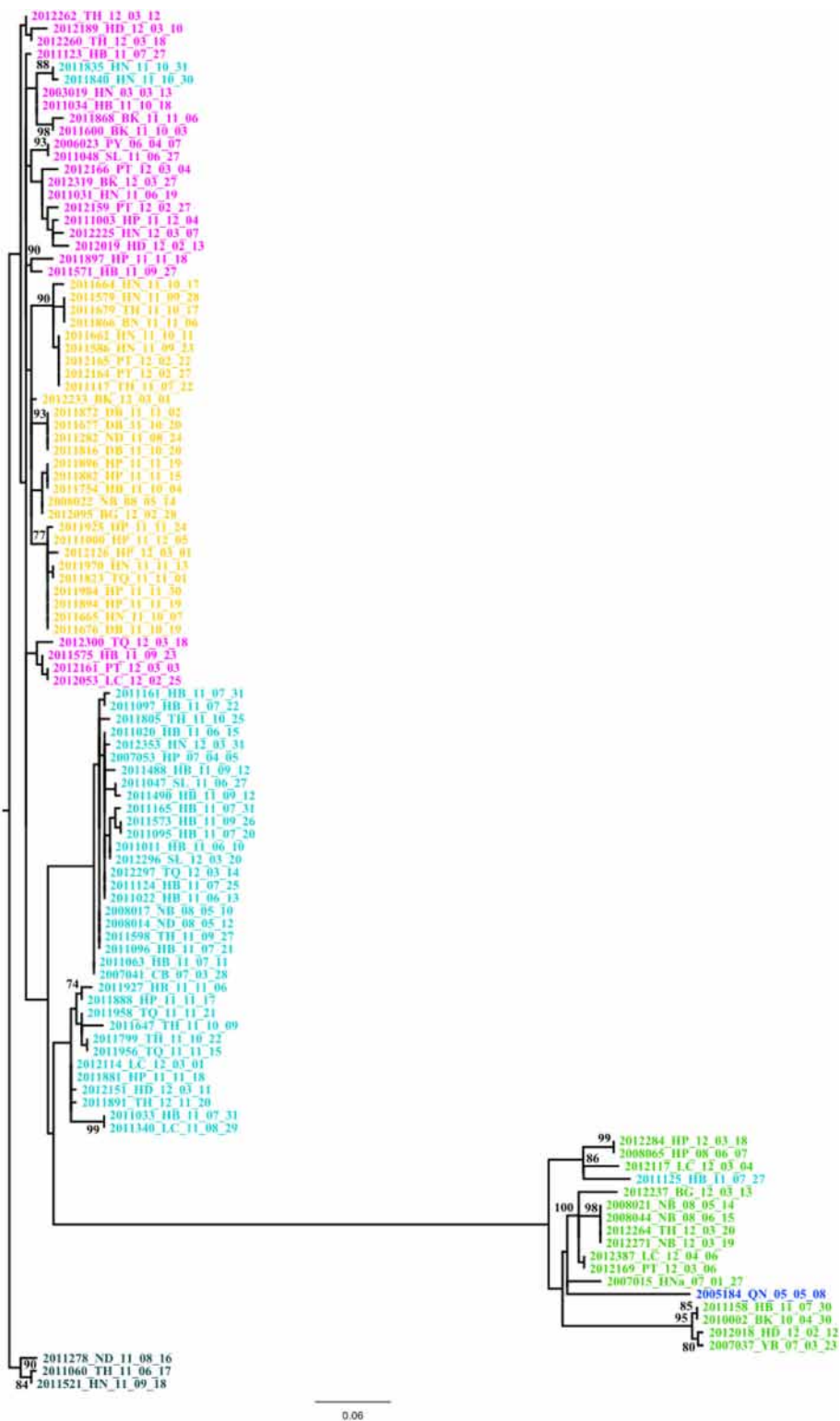
Fig. 1 Phylogenetic analysis of partial VP1 sequences. a Phylogenetic analysis of the nucleic acid sequences. Tree was designed using Maximum Likelihood. Color code: Black: VV; Light blue: VII; Yellow: IIV; Purple: VIV; Dark blue: VI
