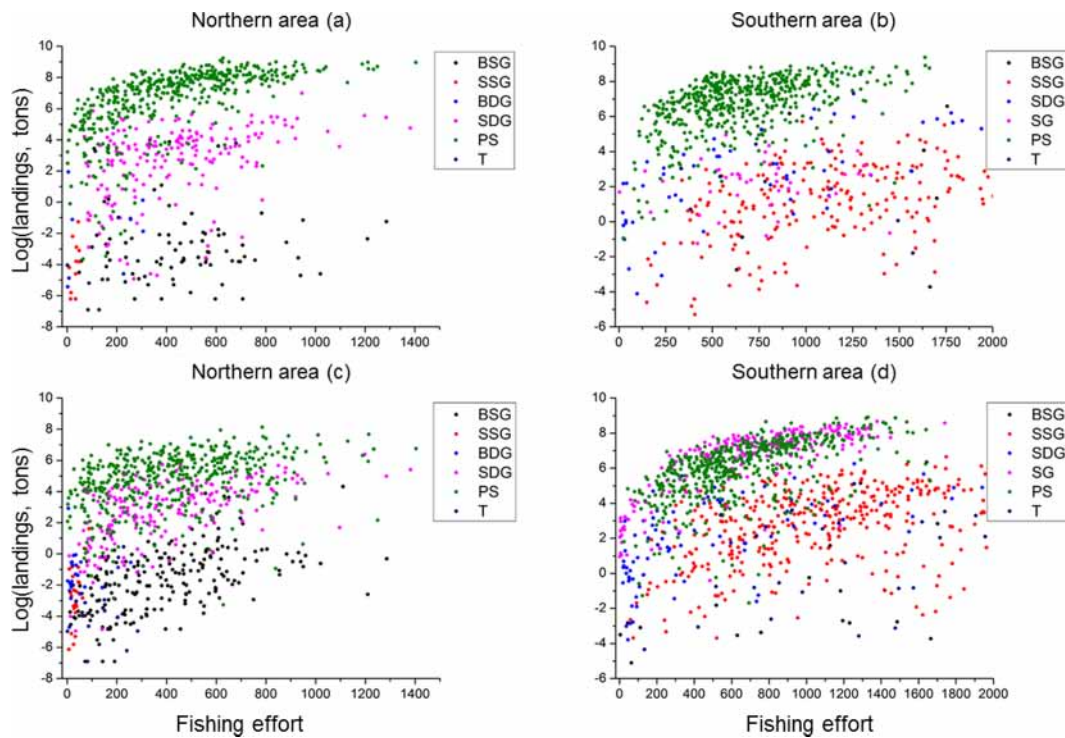
Fig. 3. Relationship between monthly landings of Sardinella aurita (a, b) and Sardinella maderensis (c, d) and fishing effort (number of trips) by fishing gear in the northern and southern area in Senegalese waters (2004–2013).
