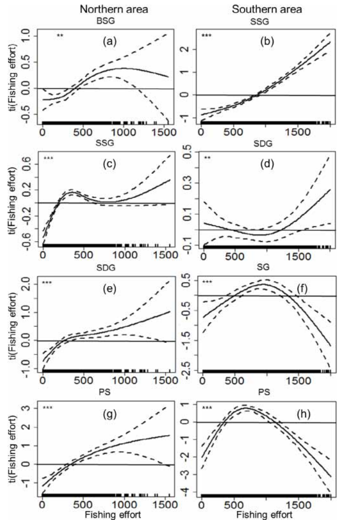
Fig. 5. Estimated smooth curves obtained by the GAM applied to landings of Sardinella maderensis in the northern area (first column) and the southern area (second column): bottom set gillnet (BSG, a); surface-set gillnet (SSG, b and c); surface-drift gillnet (SDG, d and e); surrounding gillnet (SG, f) and purse seine (PS, g and h). Dashed lines represent two standard error boundaries around the covariate main effects. Significance codes: ***0.001; **0.01; *0.05. The x-axis shows the density of points for each covariate and the y-axis reflects the relative importance of each covariate.
