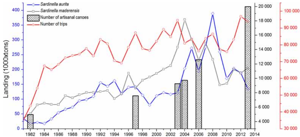
Fig. 1. Annual landing (tons) of Sardinella and fishing effort for the small-scale fishery in Senegal from 1981 to 2013. Landing of Sardinella aurita (blue line with lozenges) and S. maderensis (gray line with squares) and fishing effort (red line with circles) were extracted from the CRODT database. The number of canoes for 1982, 1997, 2003, 2004 and 2006 were obtained from the FAO (2008) and for 2013 from Belhabib et al. (2014).
