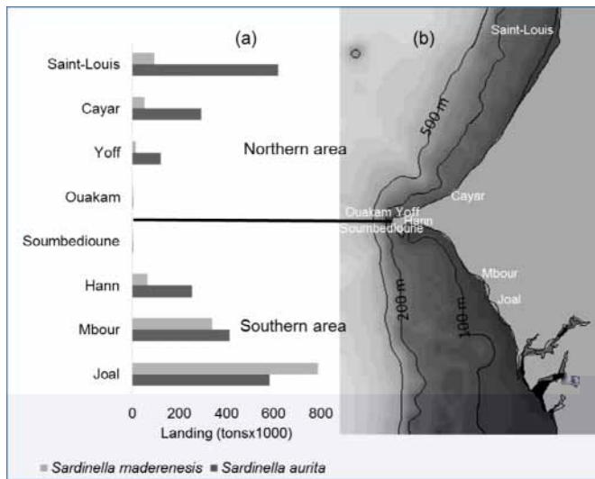
Fig. 2. (a) Total landing of Sardinella aurita (black bars) and S. maderensis (gray bars) by landing port summed over the period 2004–2013. (b) Map of landing ports along the Senegalese coast. The artisanal fleet operates generally within the area limited by the 500 m isobaths.
