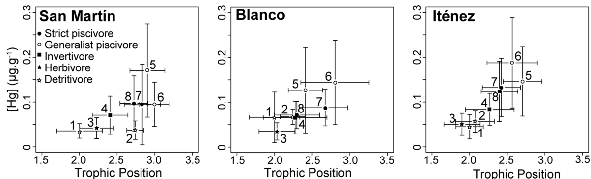
Figure 3. Mercury biomagnification in fish assemblage of three rivers from the Iténez basin (Amazon, Bolivia). Biplots display mean values ( \pm sd in error bars) of Trophic Position (derived from \delta^{15}\text{N} ) and [\text{Hg}]_{\text{ww}} of detritivore (1 = Curimatella cf. alburna , 2 = Psectrogaster sp.), herbivore (3 = Schizodon fasciatus ), insectivore (4 = Triportheus angulatus ) and piscivore (5 = Pseudoplatystoma sp., 6 = Pygocentrus nattereri , 7 = Hoplias malabaricus and 8 = Acestrorhynchus sp.) fish species. Slope of the relation correspond to biomagnification along the food chain.
