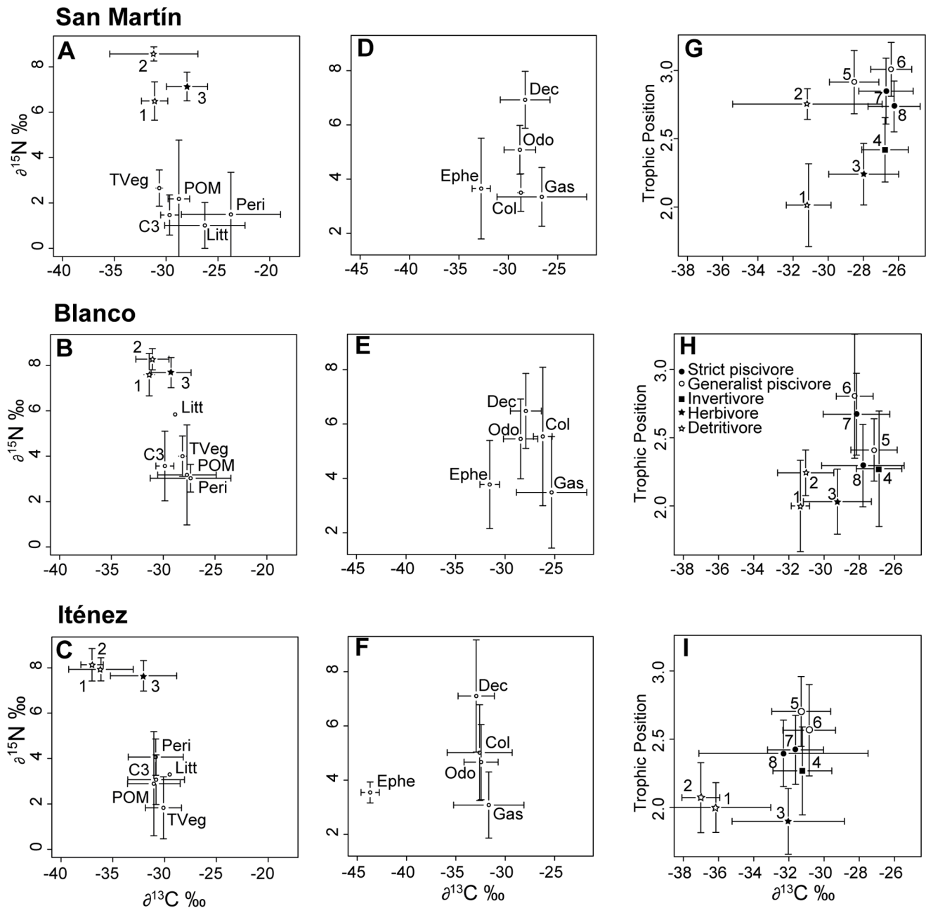
Figure 2. Isotopic signature of sources, invertebrates and fish in three rivers of the Iténez basin (Amazon, Bolivia). Biplots display mean values ( \pm sd in error bars) of \delta^{13}\text{C} and \delta^{15}\text{N} values for sources (A,B,C) POM = Particulate organic matter, Litt = Leaf litter, Peri = Periphyton; C3 = C3 aquatic macrophytes and TVeg = Terrestrial Vegetation; and invertebrates groups (D,E,F): Ephe = Ephemeroptera, Odo = Odonata, Dec = Decapoda, Col = Coleoptera and Gas = Gasteropoda. (G,H,I) represented mean values ( \pm sd in error bars) of \delta^{13}\text{C} and Trophic Position (derived from \delta^{15}\text{N} ) of fish species: detritivore (1 = Curimatella cf. albuna , 2 = Psectrogaster sp.), herbivore (3 = Schizodon fasciatus ), insectivore (4 = Triporthus angulatus ) and piscivore (5 = Pseudoplatystoma sp., 6 = Pygocentrus nattereri , 7 = Hoplias malabaricus and 8 = Acestorhynchus sp.). In biplots (A,B,C), C4 aquatic macrophytes ( \delta^{13}\text{C} : -12.3 to -13.2\text{‰} ; \delta^{15}\text{N} : 2 to 2.2\text{‰} ) were not plotted and \delta^{13}\text{C} and \delta^{15}\text{N} values of detritivore (1, 2) and herbivore (3) fish species were reported. doi:10.1371/journal.pone.0065054.g002
