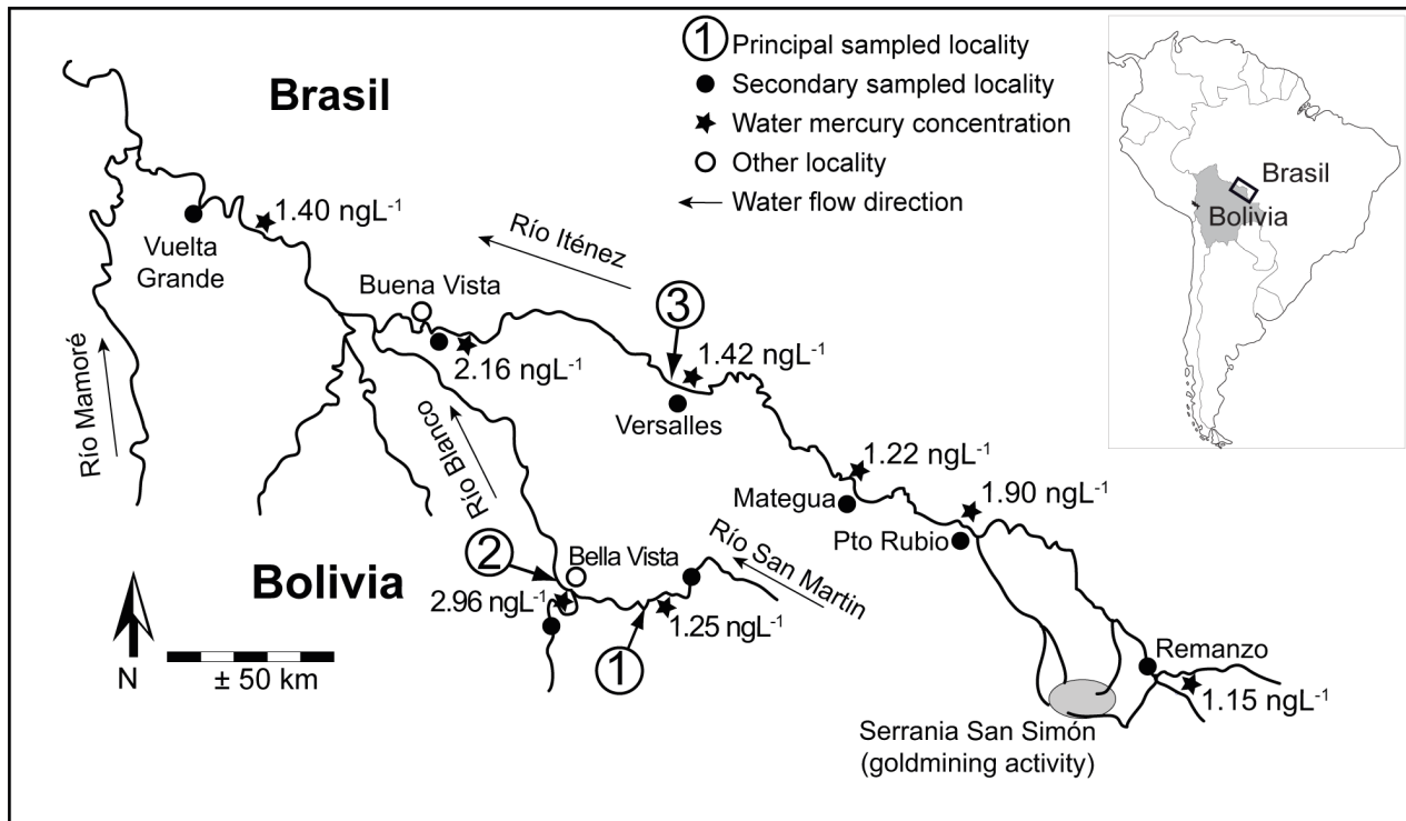
Figure 1. Hydrological map of the Bolivian part of the Iténez basin. Sampling locations (black point) and water mercury concentrations (star) are indicated. The principal sampled locations were: 1- San Martín River; 2- Blanco River; 3- Iténez River. (Redrawn from [13]). doi:10.1371/journal.pone.0065054.g001
