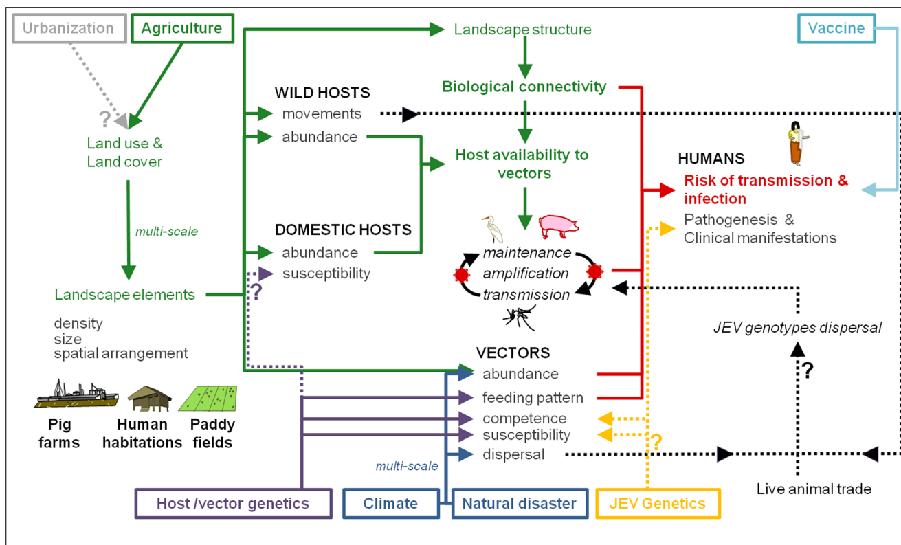
Figure 1. Overview of the drivers of the JEV ecology and epidemiology. Arrows from one driver (ex: climate) to another (ex: vectors abundance) illustrate the influence of the first on the second. Lines are dotted when the link between two drivers is uncertain. Question tags underscore uncertain aspects of the JEV cycle. The JEV is represented in red in the zoonotic cycle in the middle of the figure. Humans, as they stay outside of the JEV cycle, do not enter the cycle. Major drivers influencing the JEV ecology and ultimately the epidemiology in humans are framed. These drivers and their influences are colored as follow: in green, agriculture; in blue, climate and natural disasters; in purple, host/vector genetics; in yellow, JEV genetics; urbanization, which is a priori not relevant to the JEV life cycle, appears in gray. Vaccine, as one major nonenvironmental driver influencing the risk of JEV transmission and infection to humans, is in light blue. “multi-scale” is annotated when one driver has a multiple spatial scales effect on another. doi:10.1371/journal.pntd.0002208.g001
