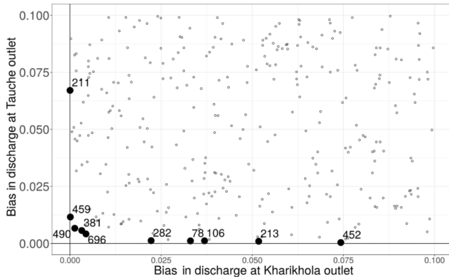
Figure 7. Scatter plot of bias in mean annual discharges for the Kharikhola and Tauche catchments for 2014–2015. Darker dots are parameter sets that provide the 10 first Pareto optima according to both criteria: bias for discharges on the Kharikhola and Tauche catchments. Optimal value for bias is 0. Graphical window is limited.
