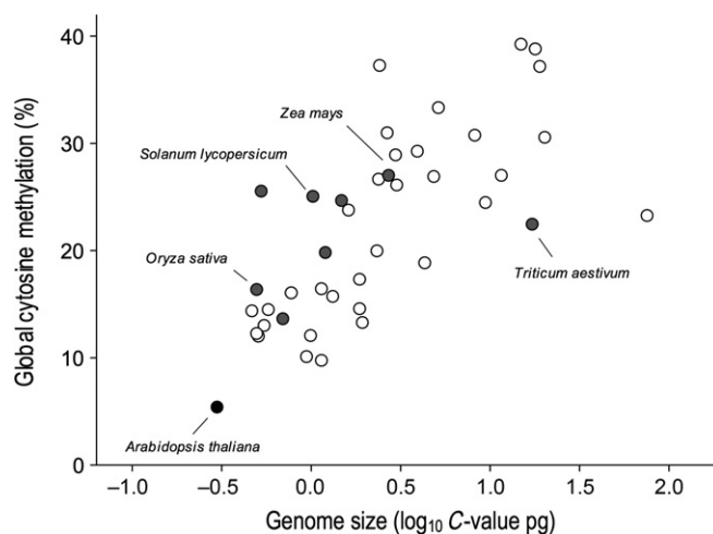
Figure 2 Features and limitations of Arabidopsis thaliana as a model system for epigenetic studies. Rapid development, selfing ability and reduced chromosome number and genome size (C-value = 0.30 pg) with relatively few repetitive and transposable elements, facilitate experimentation and simplify molecular analyses in A. thaliana . However, A. thaliana (black dot) is unusual within the range of variation in genome size and global cytosine methylation in study species, including some with a fully sequenced reference genome (filled dots) like rice ( Oryza sativa ), tomato ( Solanum lycopersicum ), maize ( Zea mays ) and wheat ( Triticum aestivum ). Redrawn from Alonso et al. (2015).
