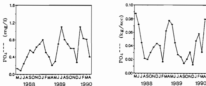
Figure 4 Variations des concentrations et des charges en sulfates, chlorures, ammoniacque, nitrates et phosphates de la Garonne en fonction du débit. Concentration and load variations of sulphates, chlorides, ammonia, nitrates and orthophosphates of the river Garonne as a function of water discharge.
