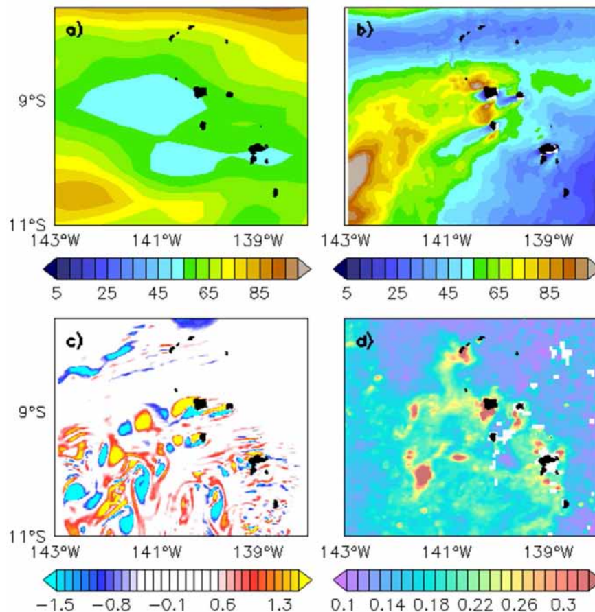
Figure 8. Annual mean of eddy kinetic energy (EKE; cm 2 /s 2 ) issued from (a) the Geostrophic and Ekman Current Observatory (GECKO) climatology with a \frac{1}{4}^\circ spatial resolution [36] and (b) a climatological 1/45^\circ resolution simulation from the Regional Ocean Modeling System (ROMS model) (see [37]); (c) Daily vorticity field ( 10^{-5}/s^1 ) at 10 m for 14 June of Year 6 from the ROMS climatological simulation; (d) Chl ( mg/m^3 ) for 20 July 2006, from the satellite-derived Chl AVE GlobColour product.
