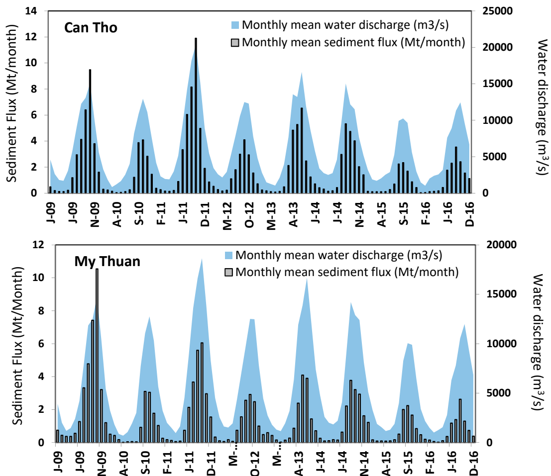
Figure 2. Evolution of monthly mean sediment flux ( \text{Mt month}^{-1} ) and water discharge ( \text{m}^3 \text{ s}^{-1} ) at CanTho (upper panel) and MyThuan (lower panel) stations during the 2009–2016 period.
