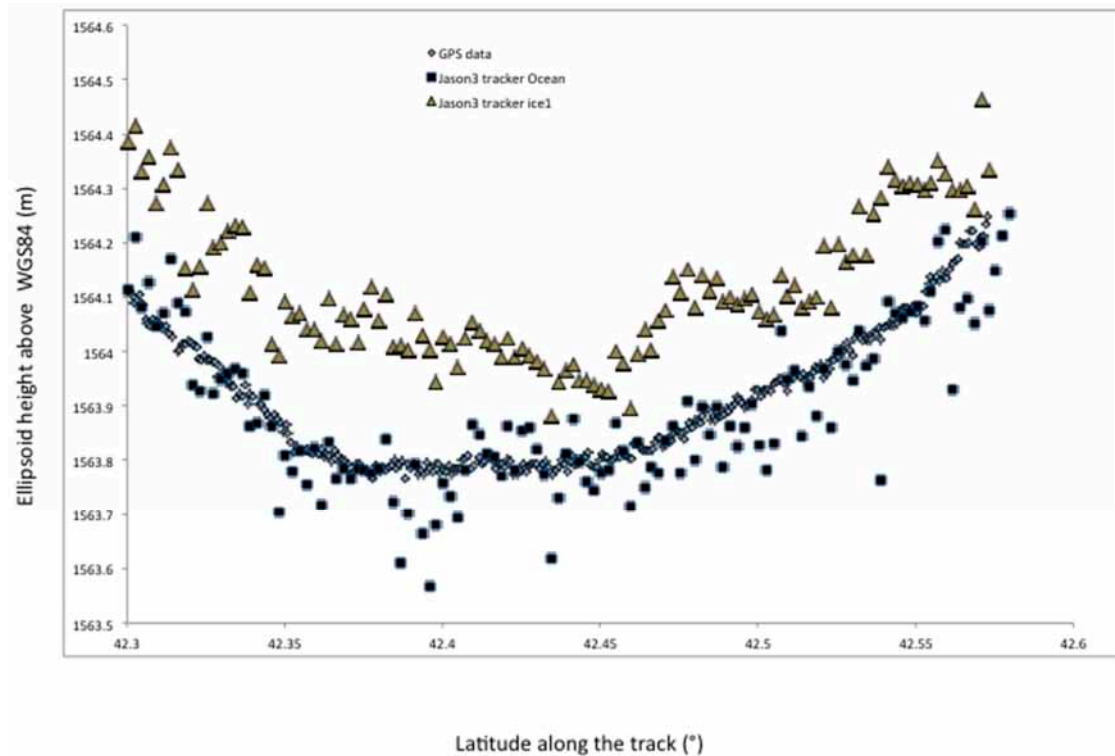
Figure 7. Ellipsoidal height of the lake surface for Jason-3 with the Ocean and Ice-1 retracker, cycle 52 (July 2017) of track 131, and shipborne measurements.
