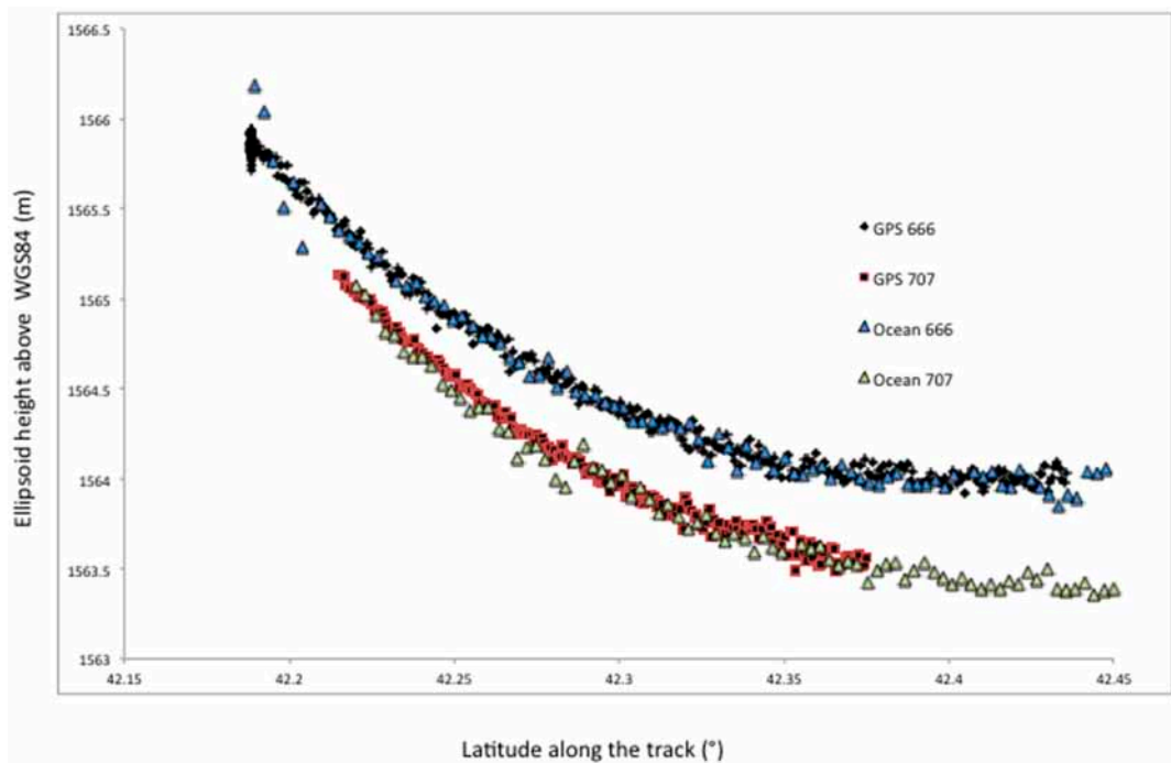
Figure 5. Ellipsoidal height of the lake surface measured by Sentinel-3A with the Ocean retracker for cycle 9 (October 2016), for the two tracks (666 and 707) and with the boat instruments.
