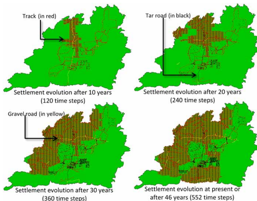
Figure 7: The settlement process over time in the Dayuma water catchment (time range: 1970 until 2016). Rectangles are colonos' fincas while polygons are limits of indigeneous comunas
