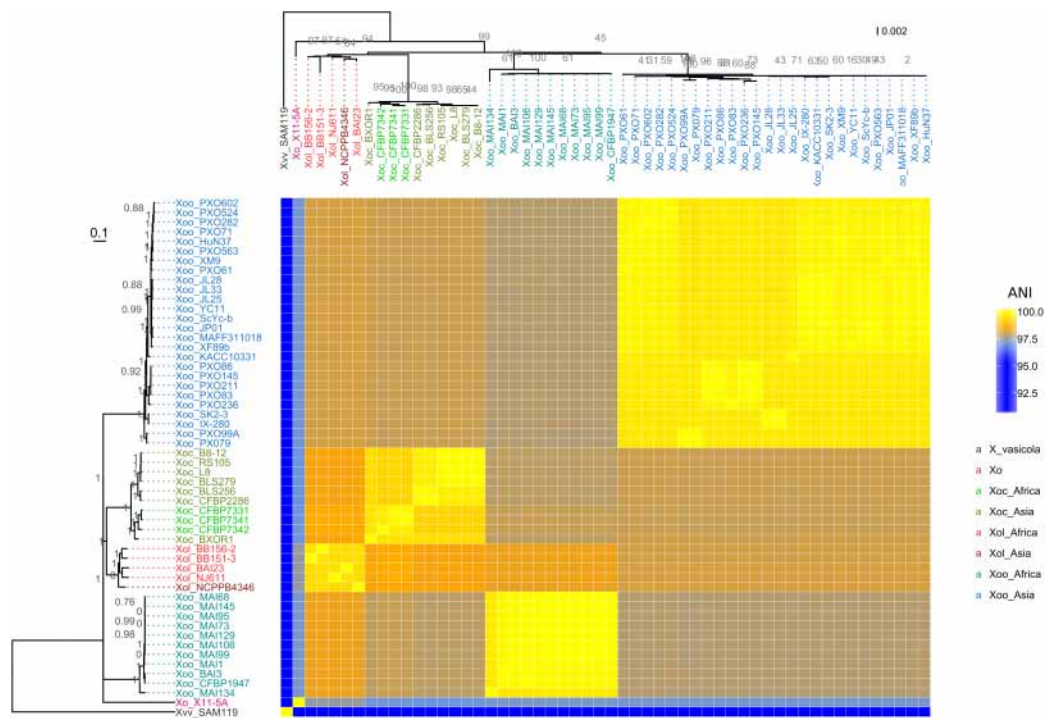
FIGURE 3 | X. oryzae pv. leersiae (Xlo) is a member of X. oryzae (Xo) and is closely related to X. oryzae pv. oryzicola (Xoc). The heatmap shows pairwise average nucleotide identity (ANI) values between fully sequenced X. oryzae genomes. (Left) Consensus parsimony tree generated with based on shared pangenome SNPs, numbers in gray indicate node support as outputted by kSNP3, heatmap rows are ordered according to this tree. (Top) MLSA neighbor-joining tree based on concatenated alignments of 33 housekeeping genes, numbers in gray indicate bootstrap support for branches, and heatmap columns are ordered according to this tree. X. oryzae pv. oryzicola is abbreviated as Xoo and X. vasicola pv. vasculorum as Xvv. All species abbreviations are followed by strain name.
