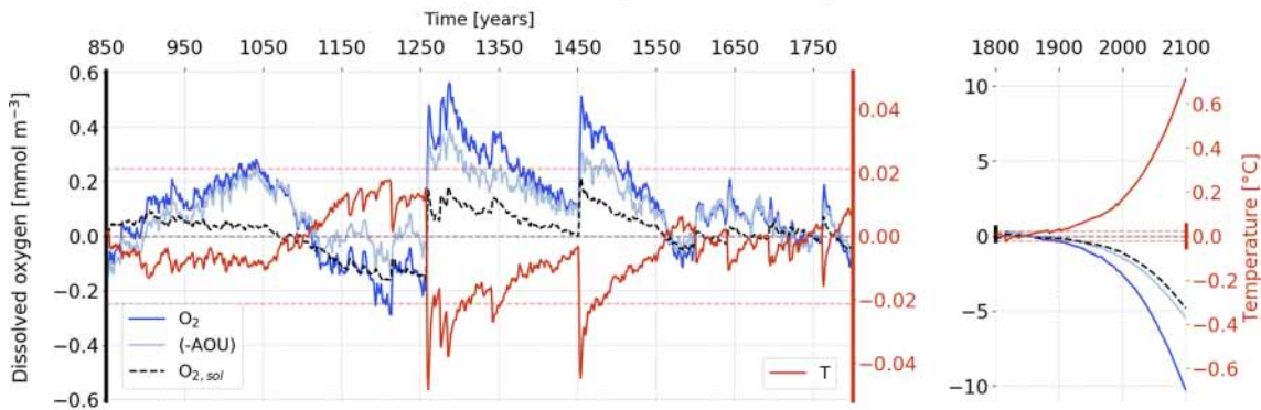
(a) Global ocean mean anomalies of oxygen, its components and temperature
