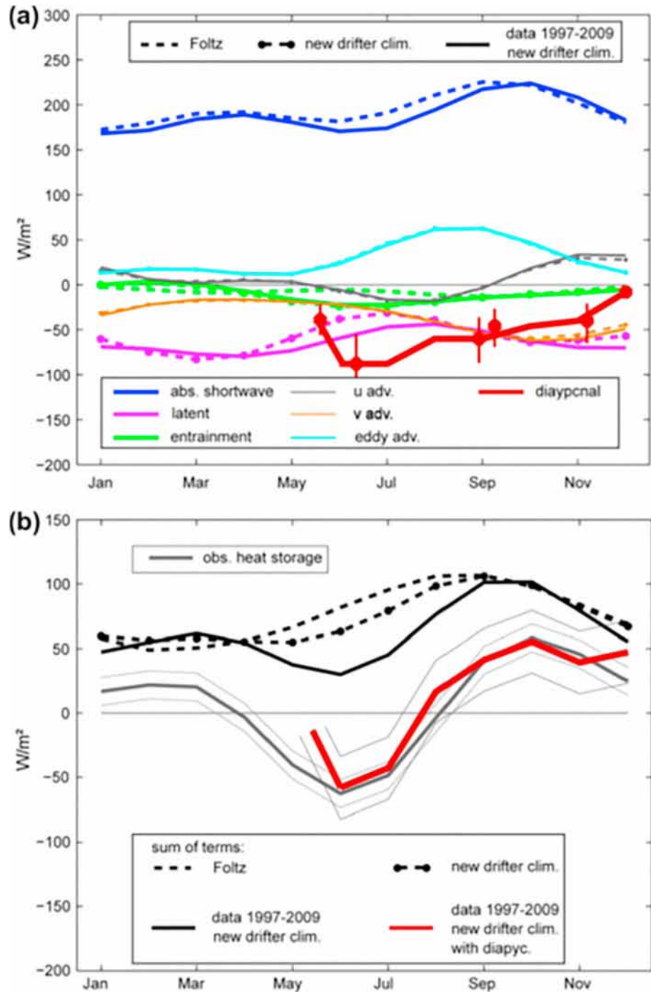
Figure 15. (a) Individual terms of the mixed layer heat budget at 10°W, 0°N: Dashed lines are a reproduction of the Foltz et al. (2003) estimates with coarse drifter resolution, using data from 1997–2002; dashed-dotted lines indicate advective and eddy heat flux estimates from the period 1997–2002 using a drifter climatology of higher resolution compared to the climatology used by Foltz et al. (2003); solid lines indicate flux estimates using the higher-resolution drifter data and data from the time period 1997–2009; the red bars denote confidence limits for the average diapycnal heat flux below the mixed layer; (b) black lines represent the sum of all terms contributing to the heat budget except turbulent heat flux (line styles are assigned to the same set ups as in (a)), red line indicates sum of all terms including diapycnal heat flux. From Hummels et al. (2013), their Figure 16 (reprinted by permission from Elsevier, License Number 4533661391935).
