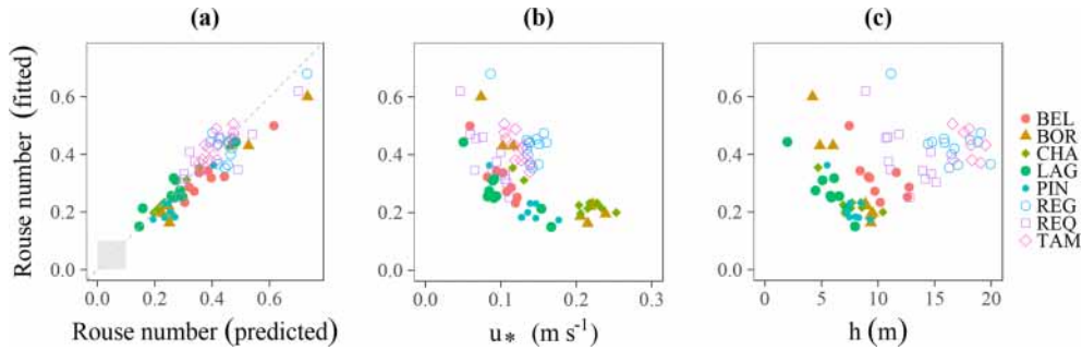
Figure 9. Fitted Rouse numbers against (a) predicted P_s (the gray square in the bottom-left represents the range of variation of P_f ), (b) shear velocities and (c) water levels.
