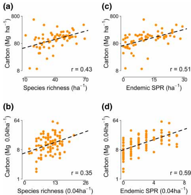
FIGURE 2 Relationships of tree species richness and endemic tree species richness with aboveground carbon storage across relatively intact and disturbed forest plots in the central Western Ghats (a, c), and Anamalai Hills (b, d). Broken lines depict predictions of simple linear regression models. Pearson's correlation coefficients ( r ) are reported
