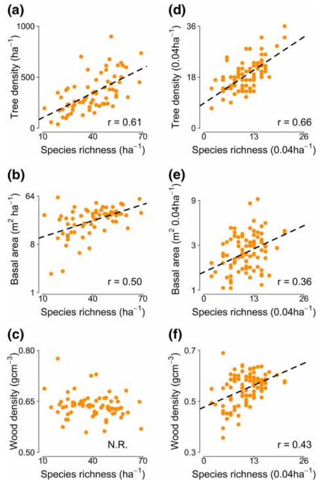
FIGURE 3 Relationships of tree species richness with tree density, basal area, and community-weighted average wood density, across relatively intact and disturbed forest plots in the central Western Ghats (a–c) and the Anamalai Hills (d–f). Broken lines depict predictions of simple linear regression models. Pearson's correlation coefficients ( r ) are reported. N.R. indicates no relationship
