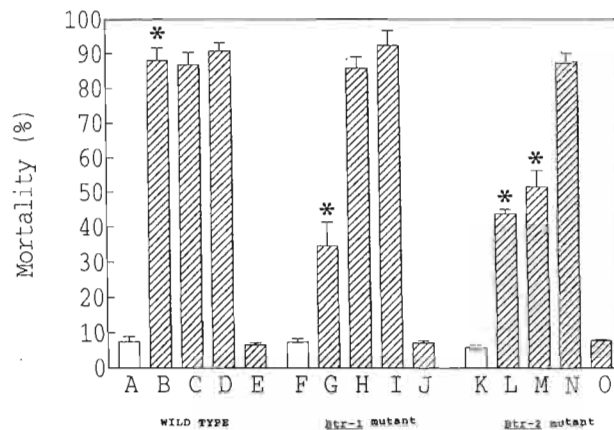
Fig. 3. Effects of different Bacillus thuringiensis strains on the mortality of Wild Type and two EMS induced mutants of C. elegans . A, F, K: control; B, G, L: Bt NRRL-18247; C, H, M: Bt 289A; D, I, N: Bt 958AB; E, J, O: Bt 302AE; for EMS induced mutants. (Data marked with an asterisk are significantly different - P < 0.001 - from the Wild Type for each Bt strain).
