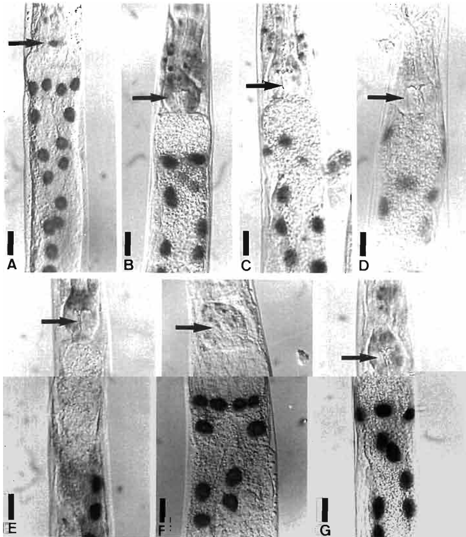
Fig. 2. Progressive destruction of intestine as result of the transgenic Caenorhabditis elegans containing the hsp-16-lacZ transgene with nematicidal Bacillus thuringiensis strain NRRL-18247. Visualisation of nuclei after a 2-h heat shock followed by \beta -galactosidase histochemistry. Incubation time- A : + 1 h; B : + 10 h; C : + 13 h; D : + 15 h; E : + 18 h; F-G : controls; F : + 24 h (PBS only); G : + 24 h, with non-nematicidal strain B. thuringiensis 302AE. Arrow indicates position of basal bulb. (Bars = 20 \mu m).
