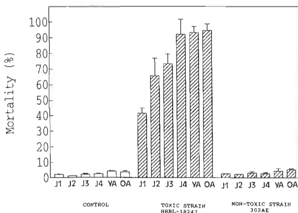
Fig. 1. Effects of nematocidal strain NRRL-18247 and non toxic strain on different Caenorhabditis elegans developmental stages. A-F: Controls (nematodes + PBS); G-L: Nematodes + NRRL-18247; M-R: Nematodes + non-toxic strain 302AE. (Incubation lasted for 24 h at 25°C; J1, J2, J3, J4 : first, second, third and fourth juvenile stage respectively; YA, OA : young and old adults respectively).
