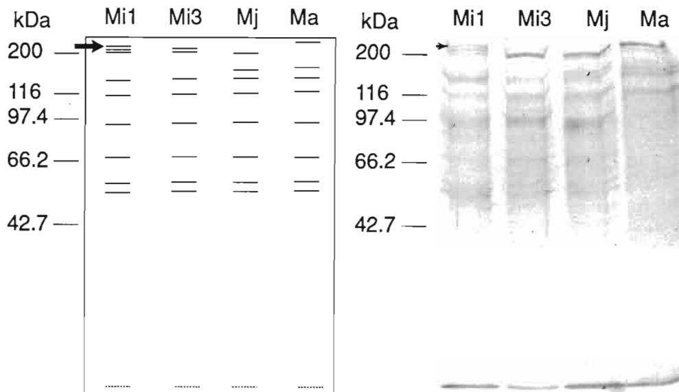
Fig. 2. Line drawing and photograph of SDS-PAGE separation of CTAB-soluble body wall extracts from second-stage juveniles of Meloidogyne spp. (13 µg protein/lane) transferred to a PVDF membrane and treated with the general protein stain, naphthol blue-black. M. incognita race 1 (Mi1); M. incognita race 3 (Mi3); M. javanica (Mj); M. arenaria race 1 (Ma). Arrow indicates a protein band unique to host race 1 of M. incognita . Electrophoretic migration of molecular weight standards is represented as kilodaltons (kDa).
