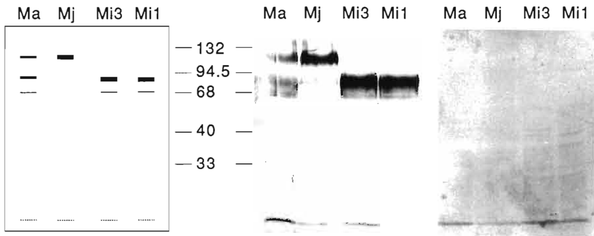
Fig. 1. Line drawing and photographs of Western blots of SDS-PAGE separation of aqueous-soluble homogenates from second-stage juveniles of Meloidogyne spp. (20 µg protein/lane) probed with (left and center) biotinylated Limulus polyphemus agglutinin and (right) biotinylated Limulus polyphemus agglutinin plus 100 mM N-Acetylneuraminic (sialic) acid. M. arenaria race 1 (Ma); M. javanica (Mj); M. incognita race 3 (Mi3); M. incognita race 1 (Mi1). Electrophoretic migration of biotinylated molecular weight standards is represented as kilodaltons (kDa).
