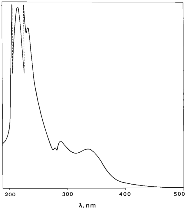
Fig. 1. UV spectrum in methanol of compound no. 6 (see Table 1) of potato cyst nematodes obtained by TLC.
