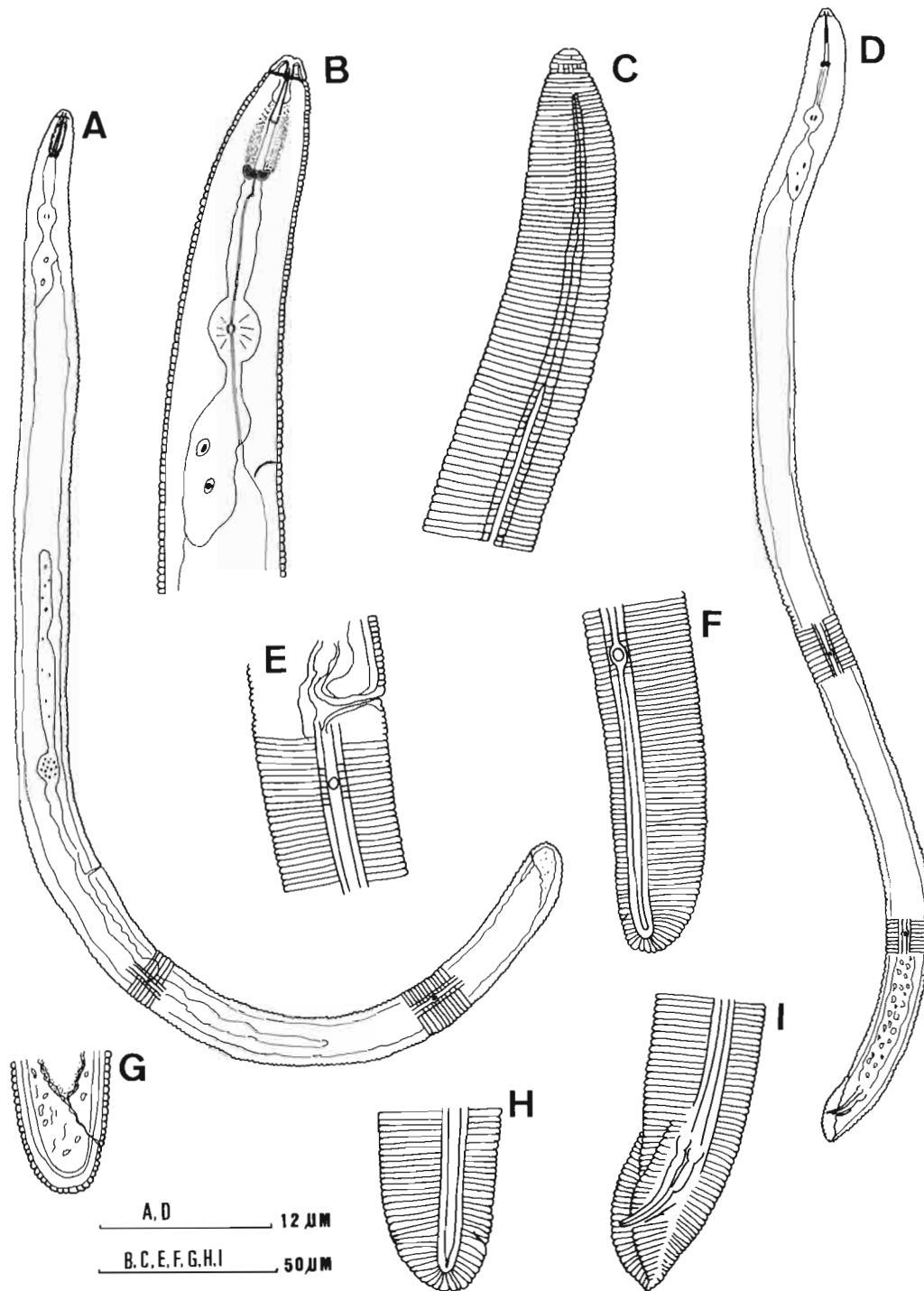
Fig. 1. Aorolaimus capsici . A : Female; B : Anterior end; C : anterior end (surface view); D : Male; E : Detail of scutellum at postvulval region; F : Posterior scutellum in female; G - H : Female tail; I : Tail of male (surface view).
