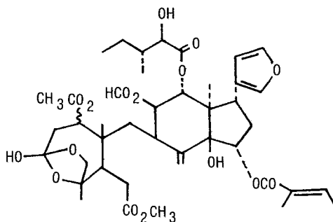
6, Hispidin A
