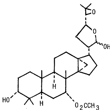
4, Glabretal
