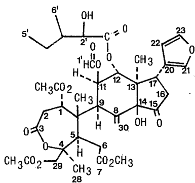
1, Prieurianin
