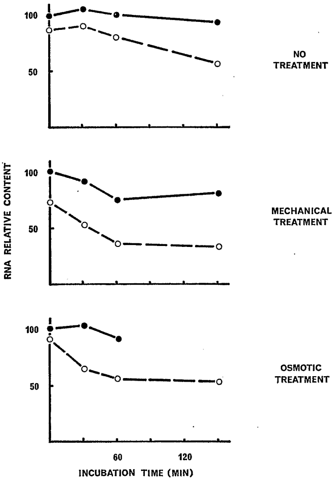
Fig. 2. Effect of pancreatic RNase on the RNA content of the lutoïd fraction. Results are expressed as percent of the initial content of the non-treated lutoïd fraction. Solid lines = untreated lutoïds; broken lines = RNase-treated lutoïds. Results represent the average of 10 experiments
