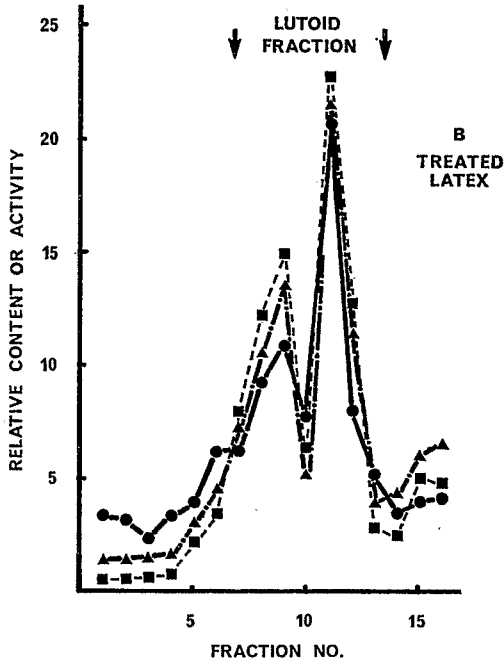
Fig. 4A and B. Influence of Neutral red on the sedimentation of lutoïds through sucrose gradient. The relative content or activity is expressed in percent of the total recovered content or activity. ■ Acid-phosphatase activity; ▲ proteins; ● RNA. (A) non-treated lutoïds, (B) lutoïds charged with Neutral red
