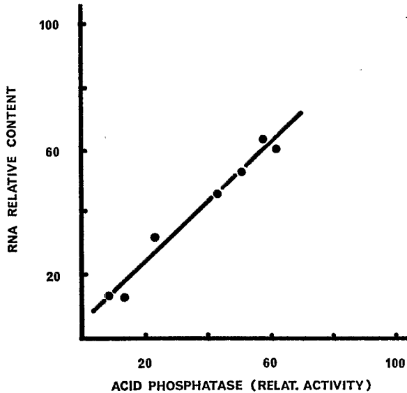
Fig. 3. Relation between RNA and acid phosphatase activity present in the sediment obtained from different destabilized lutoïd fractions by differential centrifugation. The relative RNA content and acid phosphatase activity of the 39000 \times g sediment are expressed as percent of the initial RNA content and acid-phosphatase activity of the untreated lutoïd fraction. Results represent the average of 8 experiments
