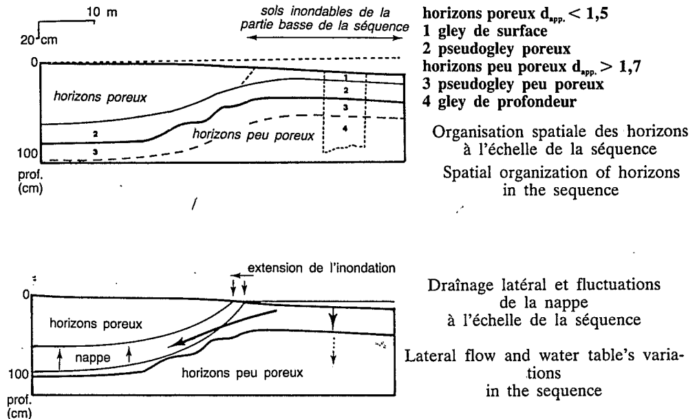
FIGURE 1. — Toposequence de Golé (plaine du Logone-Chari) Toposequence of Golé (plain of Logone-Chari)
