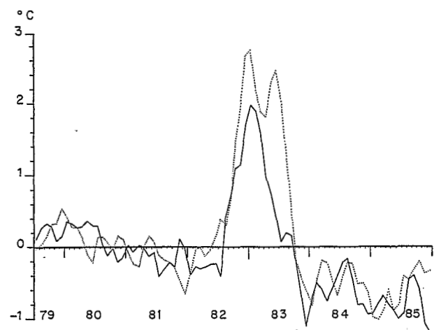
Figure 7 Eastern Pacific: mean temperature anomaly (0-300 m), 1979-1985, in degrees Celsius, integrated horizontally from the equator to 10°S (full line) and from the equator to 8°N (dotted line).
