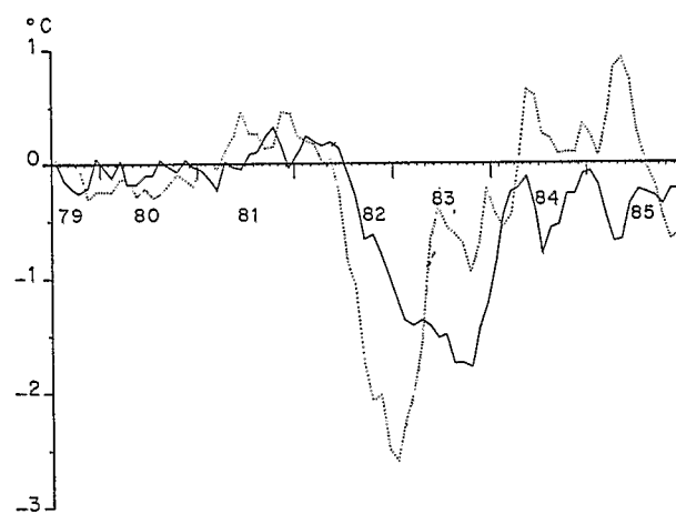
Figure 5 Western Pacific: mean temperature anomaly (0-300 m), 1979-1985, in degrees Celsius, integrated horizontally from the equator to 20°S (full line) and from the equator to 10°N (dotted line).
