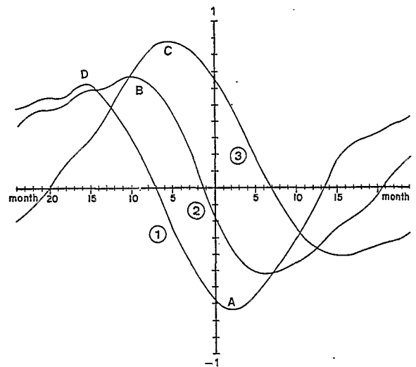
Figure 10 Cross-correlations between mean temperature anomalies (0-300 m), 1979-1985, (5°S-5°N) in the western Pacific and in the eastern Pacific (1); in the central Pacific and in the eastern Pacific (2); in the western Pacific and in the central Pacific (3). Significant correlations are denoted A, B, C, and D.
