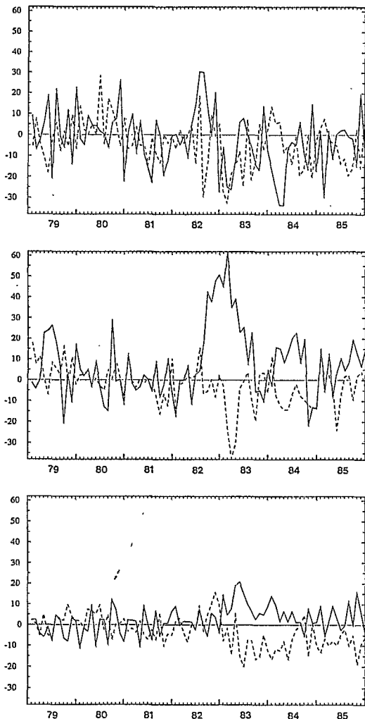
Figure 9 Wind stress anomalies at the equator: A) at 160°E, B) at 160°W and C) at 100°W (zonal component, full line; meridional component, dotted line).
