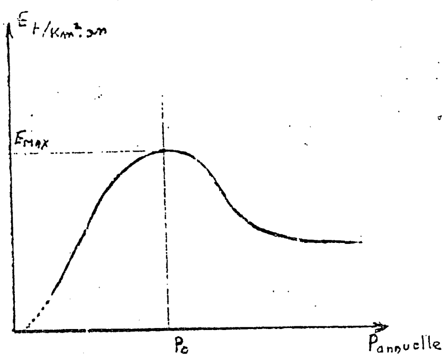
Fig 1 Erosion as a function of mean interannual rainfall
