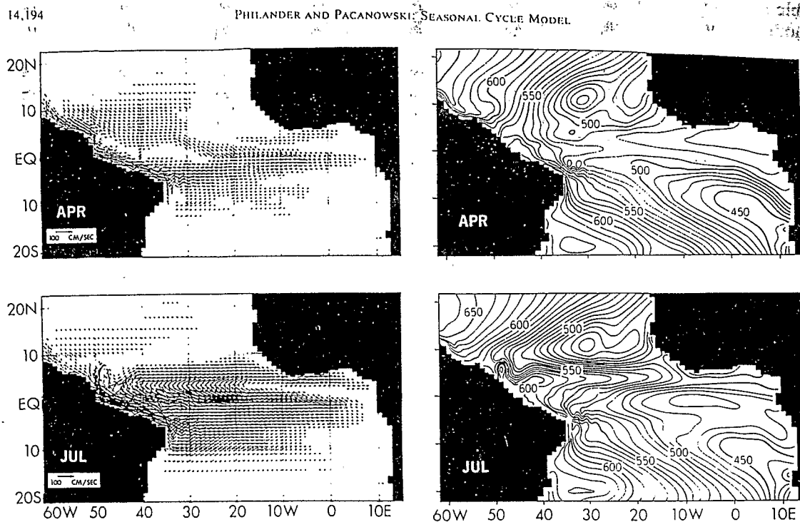
Fig. 3. Maps of surface current vectors and heat storage of the upper ocean (which is defined to be the vertical integral of the temperature from the surface to a depth of 317 m and has units of 10^3 \text{ cal cm}^{-2} ) for April 15 and July 15.
