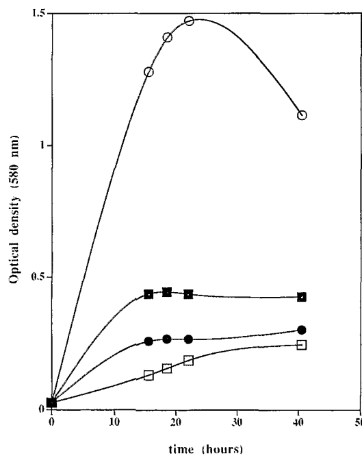
FIG. 2. Effect of electron acceptors on growth of T. maritima : ●, control; ■, S 0 (2%); □, thiosulfate (20 mM); ○, sulfate (20 mM).
