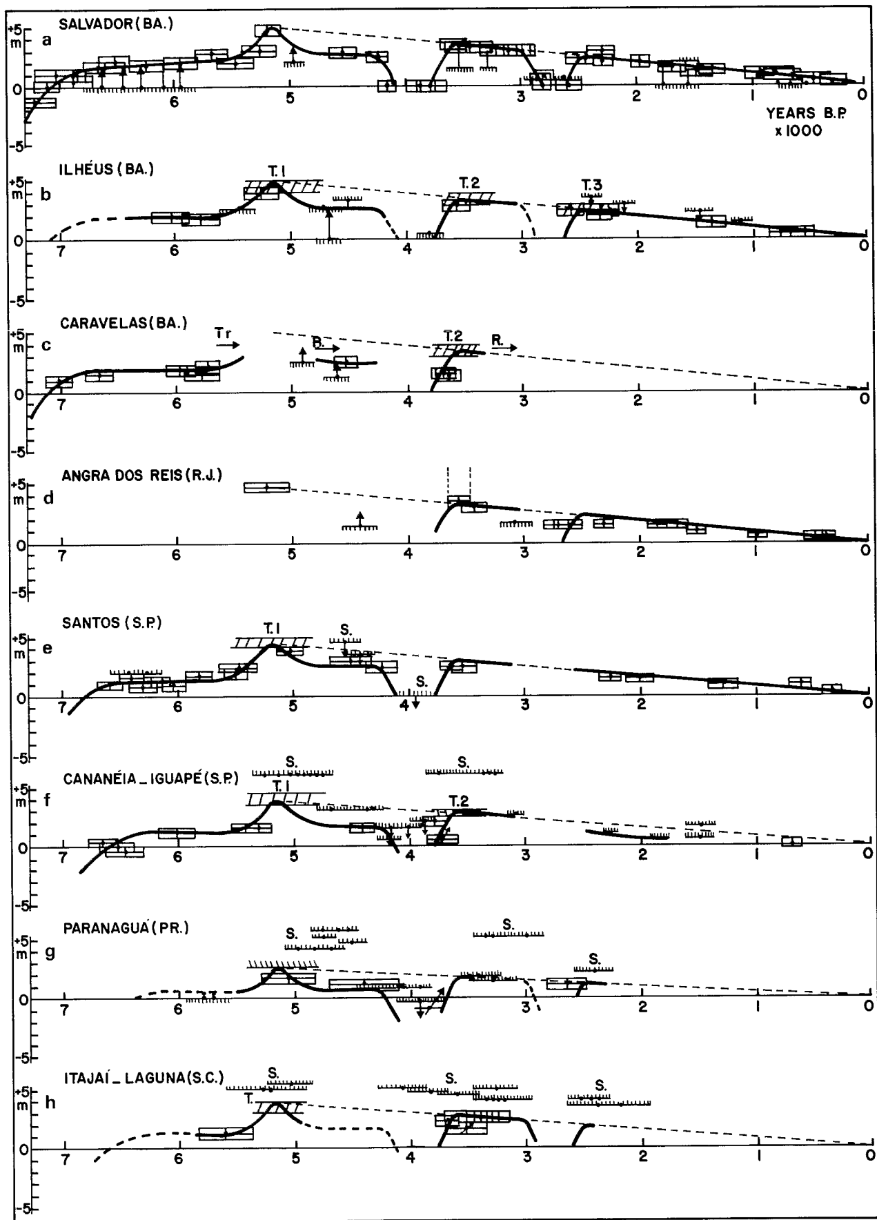
FIGURE 2 - Relative sea level fluctuation curves during the last 7,000 years for several sectors of Brazilian coast.
