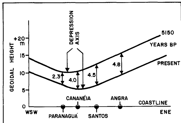
FIGURE 3 - Present day and 5,150 years B.P. geoidal surfaces. The vertical shifts can be explained by a subsidence of the geoidal relief and a slight displacement of the central depression to the east direction.
