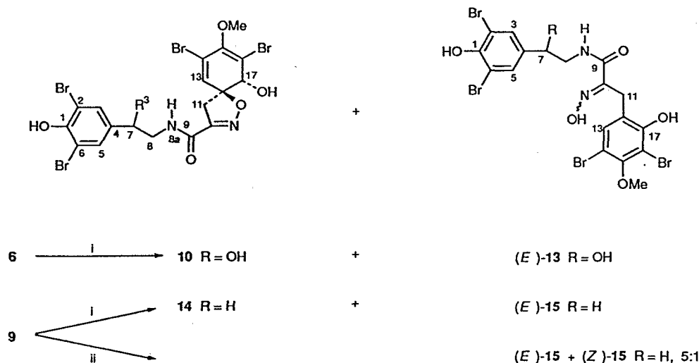
Scheme 2 Numbering is for convenience. Reagents and conditions: i, 3% KOH, MeOH, room temp., overnight; followed by acidic work-up; ii, 3% KOH, MeOH, reflux, 2 h; followed by neutral work-up.
