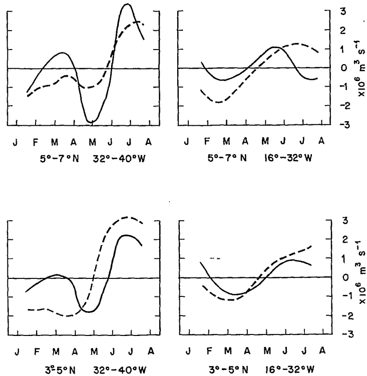
Fig. 8. Comparison between the left- and right-hand sides of equation (6). The solid lines represent y^2 h_t - c^2/\beta h_x and the dashed lines -y/\beta (\partial\tau_y/\partial x - \partial\tau_x/\partial y) - \tau_x/\beta . The ordinate scale is in \text{m}^3 \text{s}^{-1} .
