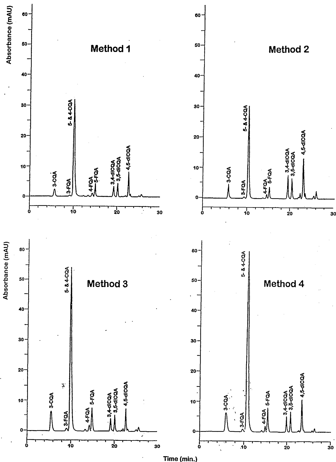
Figure 2. HPLC chromatograms of the four methods of purification of chlorogenic acids from green C. liberica var. deweyrei beans. Chromatographic conditions were as follows: solvent A, 5% methanol in 2 mM phosphoric acid; solvent B, 5% of 2 mM phosphoric acid in pure methanol; gradient A-B mixture (75/25) to pure B solvent in 45 min; column 250 × 4 mm Merck Superspher C 18 ; 10 \mu L injection; flow rate, 0.8 mL min -1 ; detection at 325 nm.
