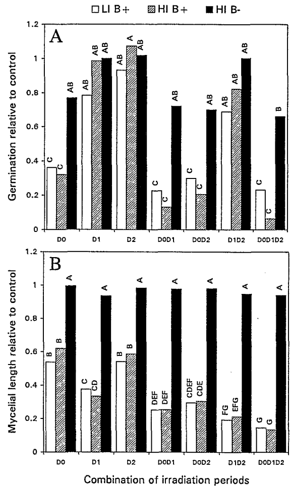
Figure 1. Effect of irradiation treatments on conidial germination (A) and mycelial growth (B) tested under solar simulation. Data recorded 72 h after inoculation. LI B+: 0.7 \text{W m}^{-2} UV B irradiance, irradiation period of 8 h; HI B+: 1.3 \text{W m}^{-2} UV B irradiance, irradiation period of 4 h; HI B-: 0.2 \text{W m}^{-2} UV B irradiance, irradiation period of 4 h. Treatments corresponding to the different combinations of irradiation period are given in Table 2. Means in each figure are based on data recorded from 7 leaf disks by treatment averaged over 2 experiments. In each figure, bars labeled with the same letter are not significantly different from each other according to Student-Newman-Keuls multiple range test ( P = 0.05 ).
