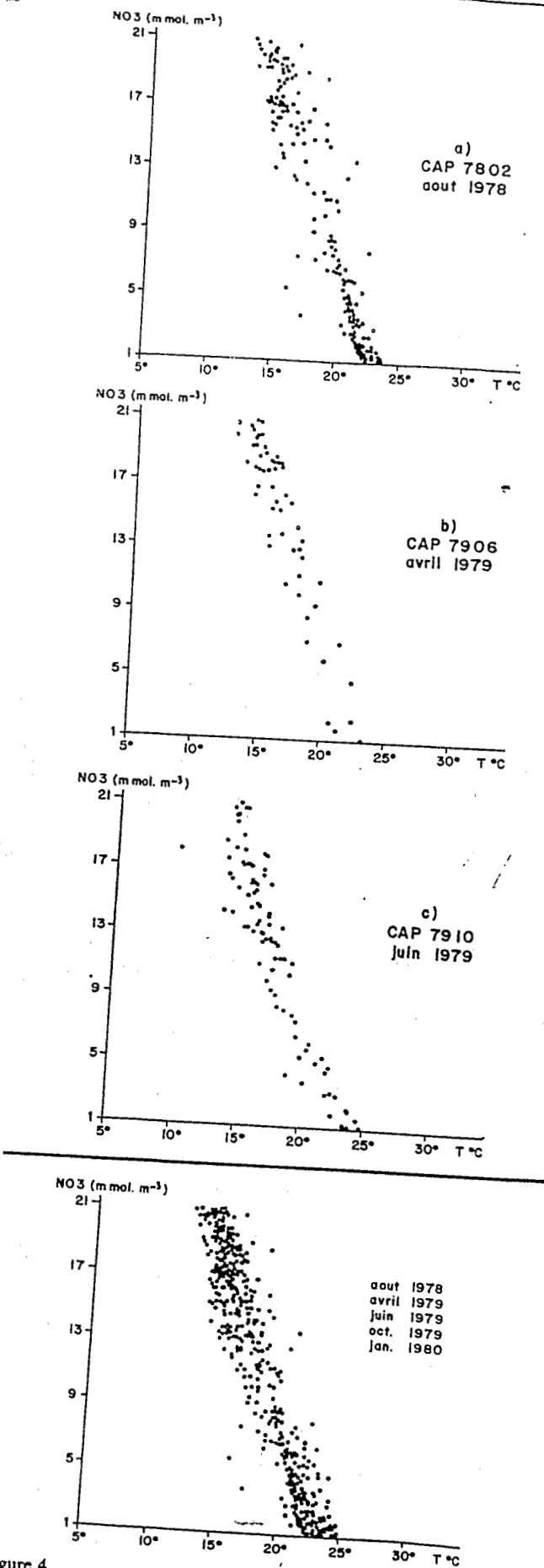
Figure 4 Relation nitrate/température le long de 4°W entre 0 et 5°S pendant le programme Cipea toutes croisières confondues. Relationship nitrate/temperature along 4°W between 0 and 5°S during the Cipea programme independent of the season.
