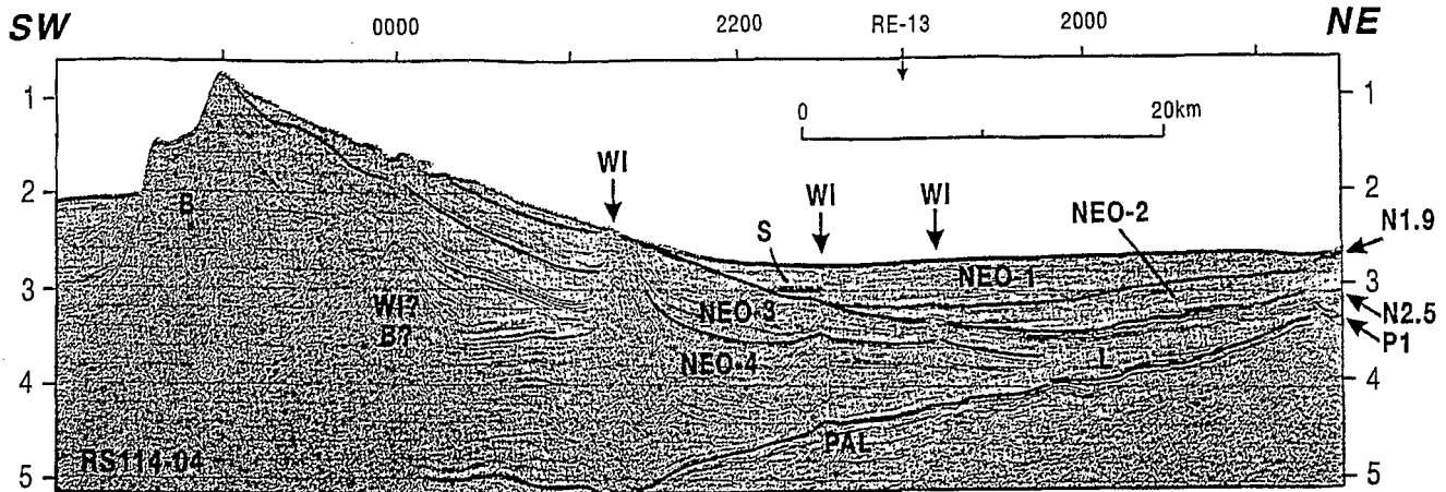
Fig. 14 [RS114-04]. Seismic reflection detail of the Wanganella Ridge and East Wanganella Sub-basin. The strong divergence of two main sedimentary packages in the Neo-4 sequence indicates two pulses of rapid subsidence probably controlled by a major listric normal fault located under the present ridge with a basin hinge line near the right-hand side of the profile. The lens of sediment (L) at right above the strong southwest-dipping P1 reflector suggests that subsidence began sometime after the development of P1 (in the very late Oligocene or very early Miocene?). Lens L is of local extent only and we include it in Neo-4. Subsidence had probably halted before the Middle Miocene as sequence Neo-3 does not have the dramatic wedge shape of Neo-4. Rather, passive onlapping of untitled sequences Neo-2 and Neo-1 on reflector N2.5 shows that rapid eversion took place at the end of Neo-3 (middle Miocene) deposition. Substantial basement slivers (B) were thrust up during the basin eversion. The distinction between basement and sedimentary sequences is complicated by several Pliocene intrusive bodies (WI, under vertical arrows). The bodies appear to include both vertical and horizontal shapes. A short horizontal body 300 ms below the seabed under S could be a flow or thin sill.
