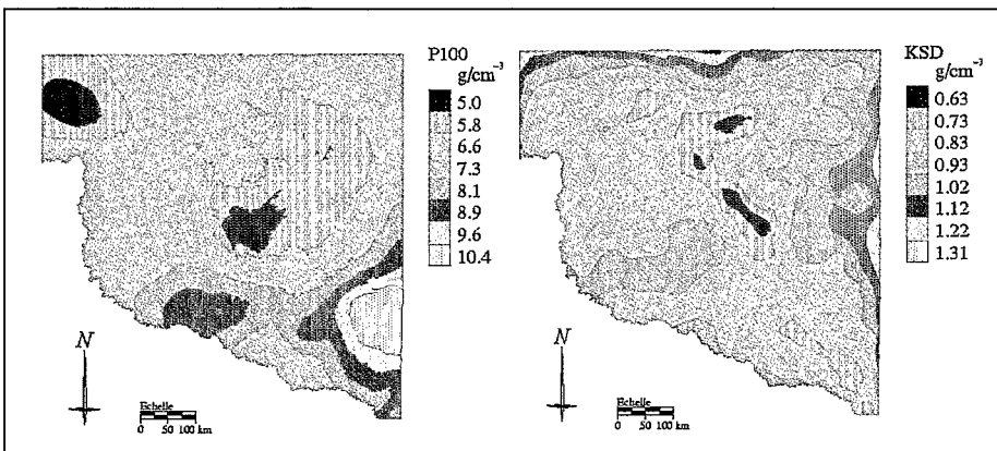
Figure 5 - Carbon stocks down to 1 m depth obtained by block kriging of punctual values (P100) and maps of associated errors (KSD).
