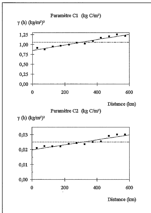
Figure 6 - Experimental variograms and fitted models for the variables C_1 and C_2 .
