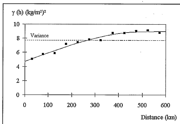
Figure 4 - Experimental variogram and fitted model for variable P100
