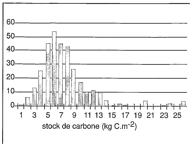
Figure 3 - Histogramme de distribution de la variable P100 Figure 3 - Frequency distribution of the variable P100
