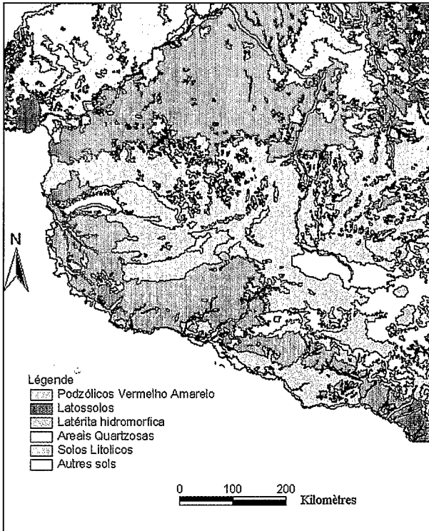
Figure 2 - Main soil map units in the study area (from 1:1 000 000 soil map)
