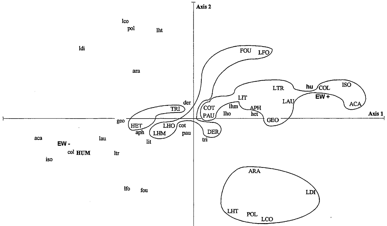
Fig. 1 Correspondence analysis (CA) on the microarthropod fauna. Projection in the plane of axes 1 and 2. For codes, see Table 2
