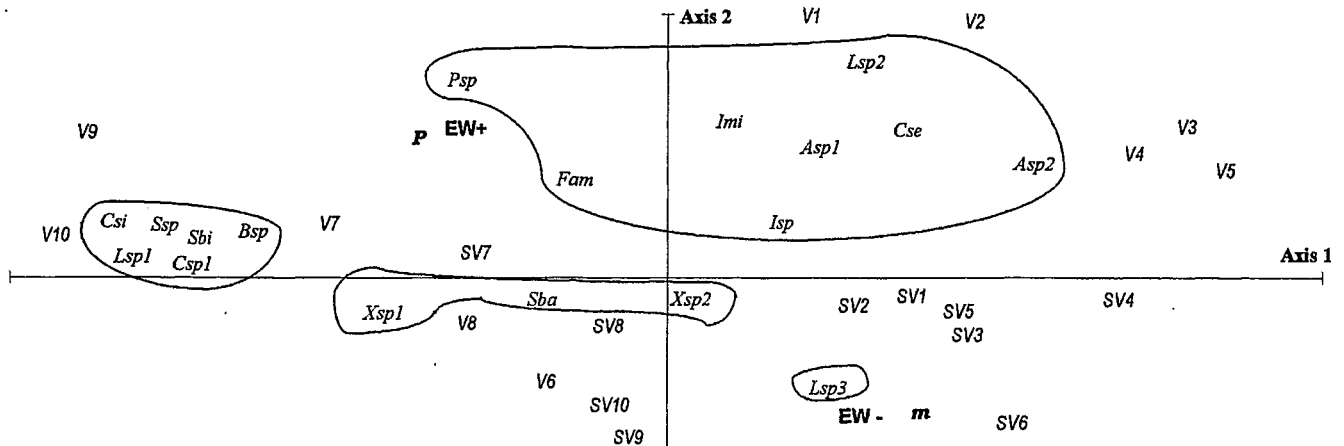
Fig. 2 CA on collembolan species. Projection in the plane of axes 1 and 2. For codes see, Table 3
