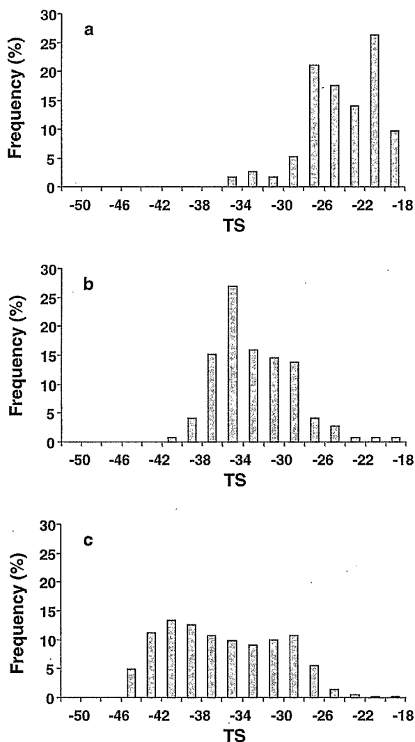
Figure 3. Distribution of TS values for the three types of aggregation: (a) 'deep scattered fish', (b) 'intermediate scattered fish' and (c) 'shallow schooling fish'.
